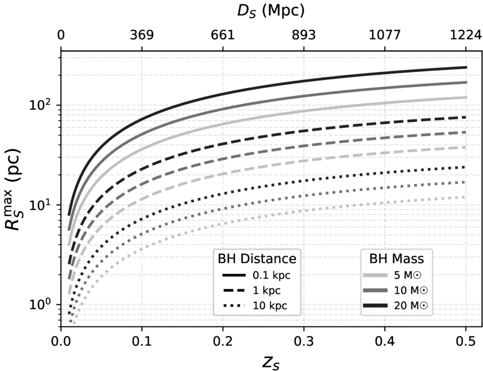
Figure 1. from Dezi Liu 2026 Astrophys. J. Lett. 1007 doi:10.3847/2041-8213/ae9306 https://dx.doi.org/10.3847/2041-8213/ae9306 © 2026. The Author(s). Published by the American Astronomical Society.
