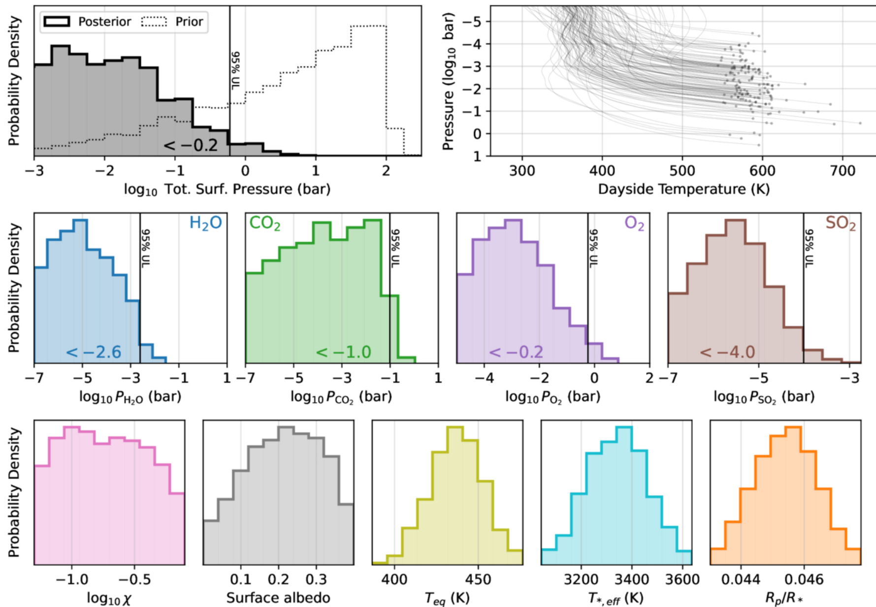
Figure 3. from Nicholas F. Wogan et al 2026 Astrophys. J. Lett. 1007 doi:10.3847/2041-8213/ae9305 https://dx.doi.org/10.3847/2041-8213/ae9305 © 2026. The Author(s). Published by the American Astronomical Society.
