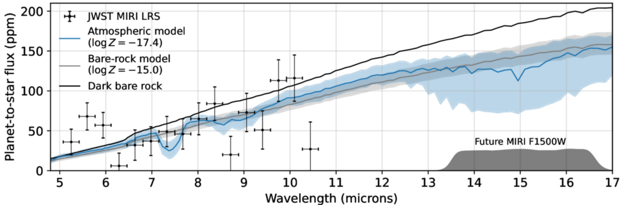
Figure 2. from Nicholas F. Wogan et al 2026 Astrophys. J. Lett. 1007 doi:10.3847/2041-8213/ae9305 https://dx.doi.org/10.3847/2041-8213/ae9305 © 2026. The Author(s). Published by the American Astronomical Society.
