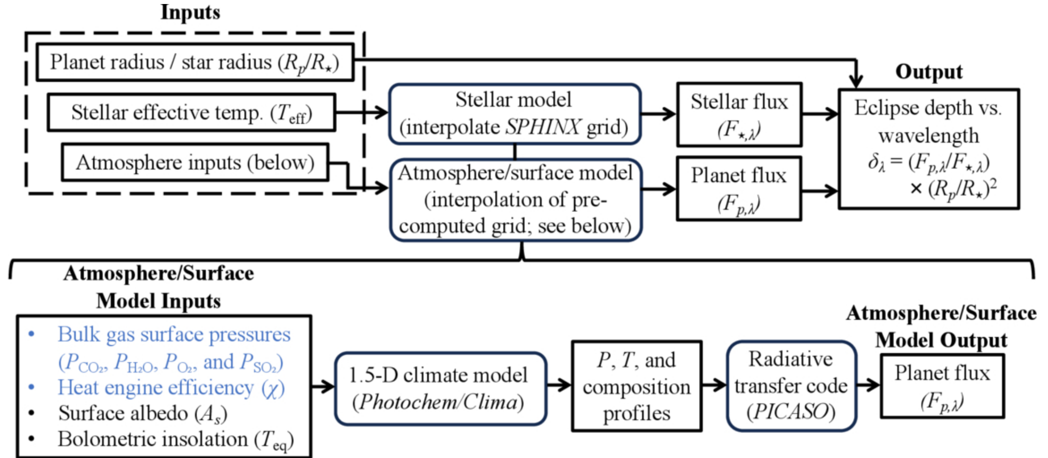
Figure 1. from Nicholas F. Wogan et al 2026 Astrophys. J. Lett. 1007 doi:10.3847/2041-8213/ae9305 https://dx.doi.org/10.3847/2041-8213/ae9305 © 2026. The Author(s). Published by the American Astronomical Society.
