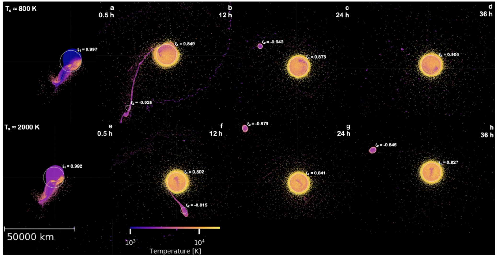
Figure 7. from C. Adeene Denton et al 2026 Astrophys. J. Lett. 1008 doi:10.3847/2041-8213/ae91e9 https://dx.doi.org/10.3847/2041-8213/ae91e9 © 2026. The Author(s). Published by the American Astronomical Society.
