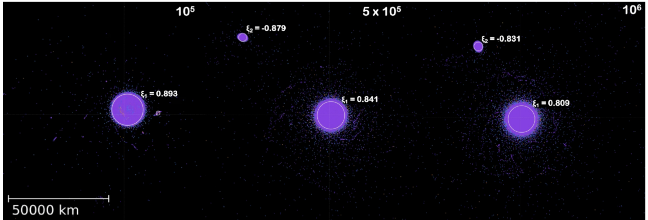
Figure 6. from C. Adeene Denton et al 2026 Astrophys. J. Lett. 1008 doi:10.3847/2041-8213/ae91e9 https://dx.doi.org/10.3847/2041-8213/ae91e9 © 2026. The Author(s). Published by the American Astronomical Society.
