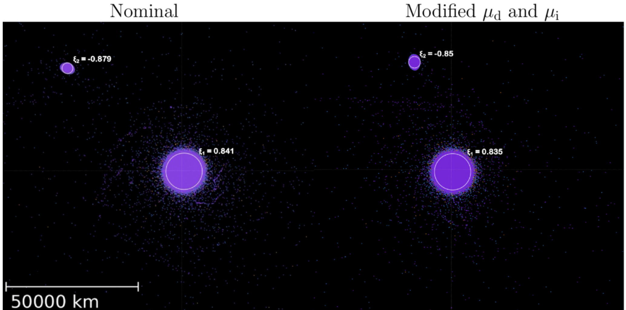
Figure 5. from C. Adeene Denton et al 2026 Astrophys. J. Lett. 1008 doi:10.3847/2041-8213/ae91e9 https://dx.doi.org/10.3847/2041-8213/ae91e9 © 2026. The Author(s). Published by the American Astronomical Society.
