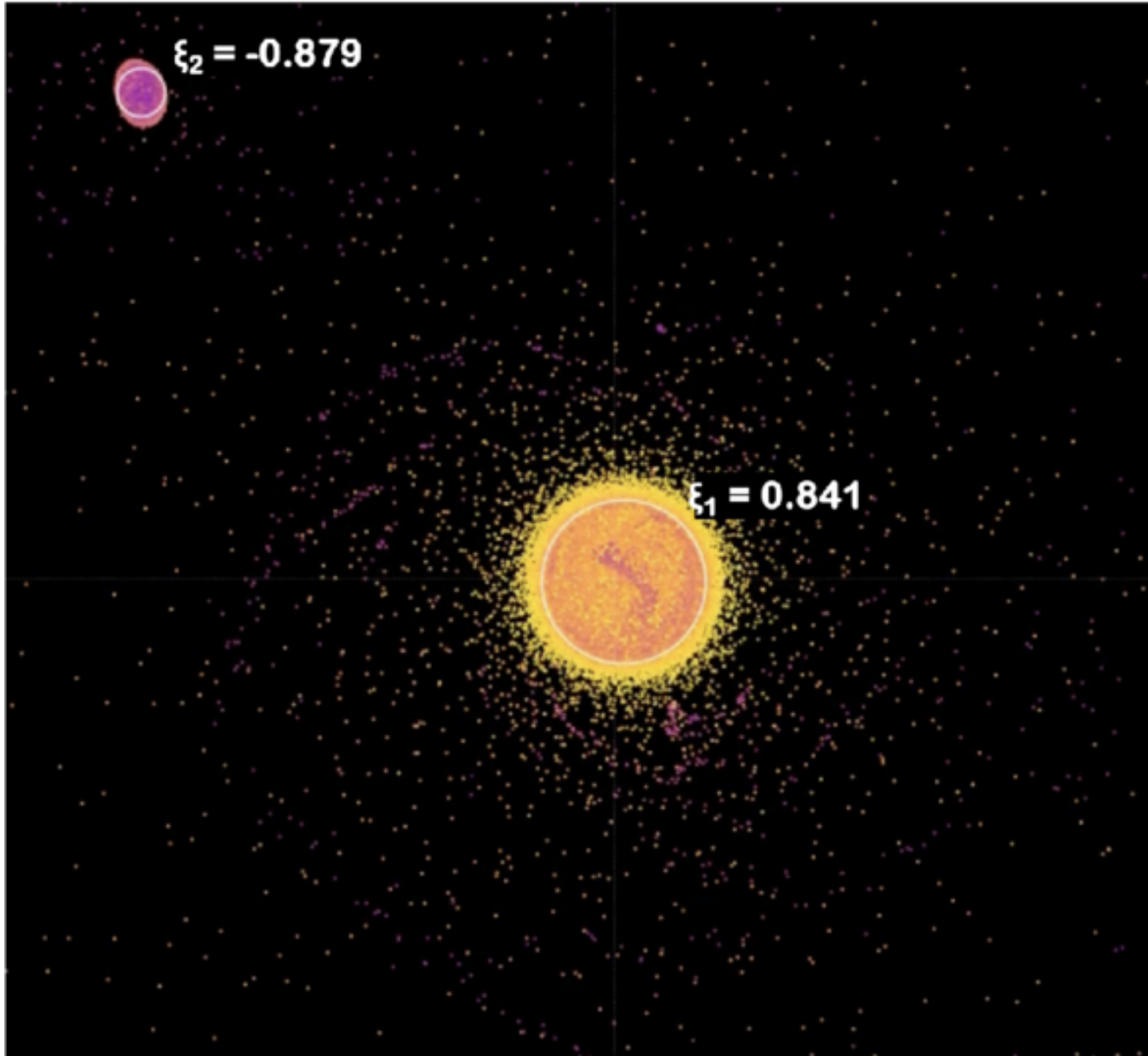
Figure 10. from C. Adeene Denton et al 2026 Astrophys. J. Lett. 1008 doi:10.3847/2041-8213/ae91e9 https://dx.doi.org/10.3847/2041-8213/ae91e9 © 2026. The Author(s). Published by the American Astronomical Society.
