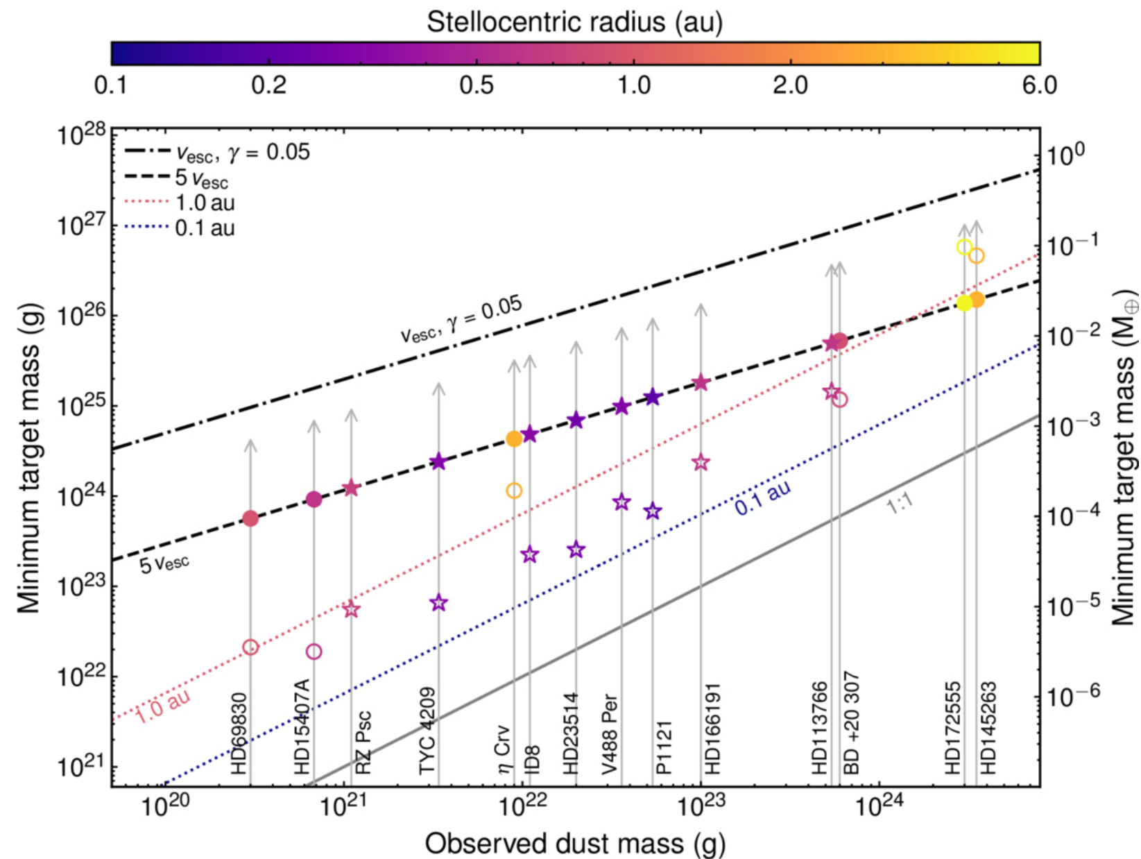
Figure 3. from Philip J. Carter and Zoë M. Leinhardt 2026 Astrophys. J. Lett. 1007 doi:10.3847/2041-8213/ae91e4 https://dx.doi.org/10.3847/2041-8213/ae91e4 © 2026. The Author(s). Published by the American Astronomical Society.
