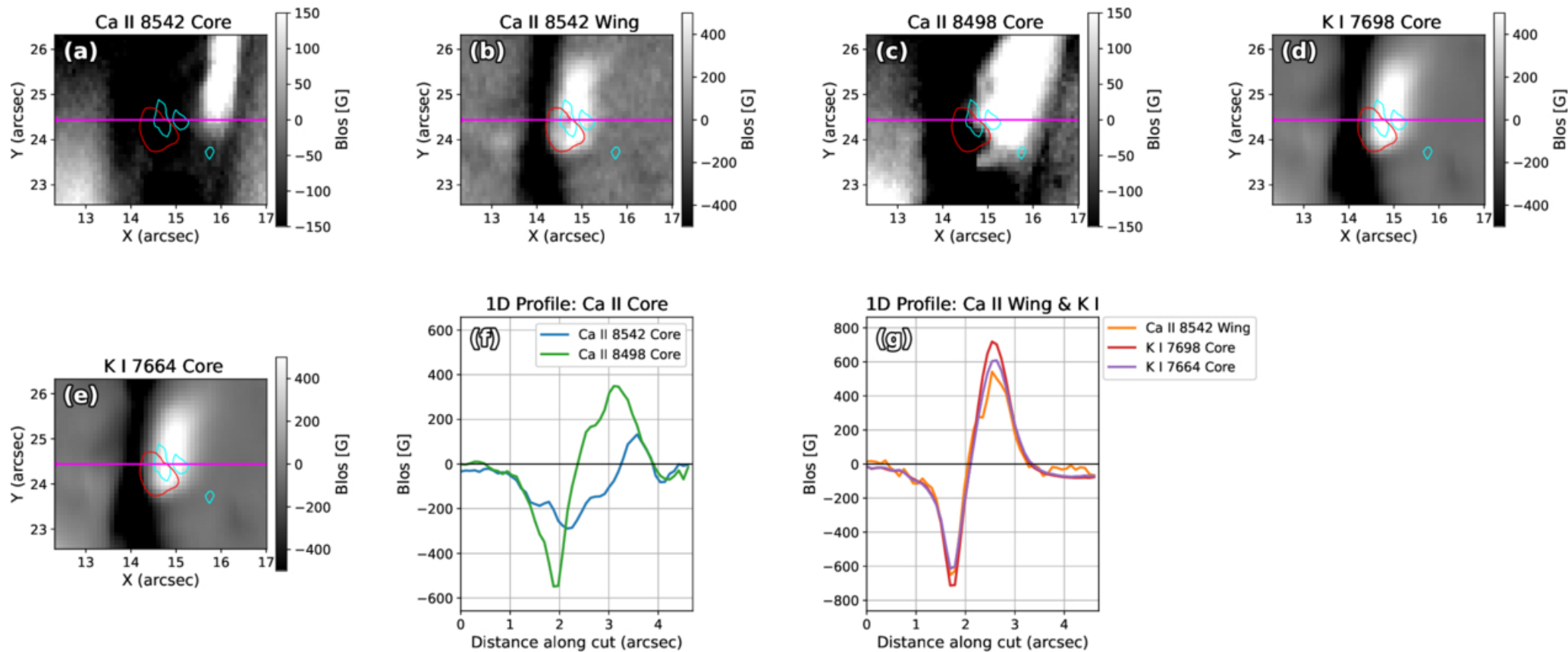
Figure 5. from Yusuke Kawabata et al 2026 Astrophys. J. Lett. 1007 doi:10.3847/2041-8213/ae91e0 https://dx.doi.org/10.3847/2041-8213/ae91e0 © 2026. The Author(s). Published by the American Astronomical Society.
