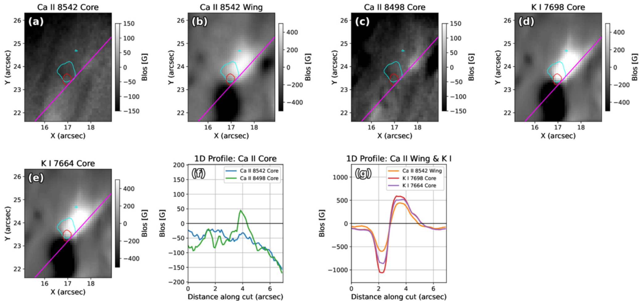
Figure 4. from Yusuke Kawabata et al 2026 Astrophys. J. Lett. 1007 doi:10.3847/2041-8213/ae91e0 https://dx.doi.org/10.3847/2041-8213/ae91e0 © 2026. The Author(s). Published by the American Astronomical Society.
