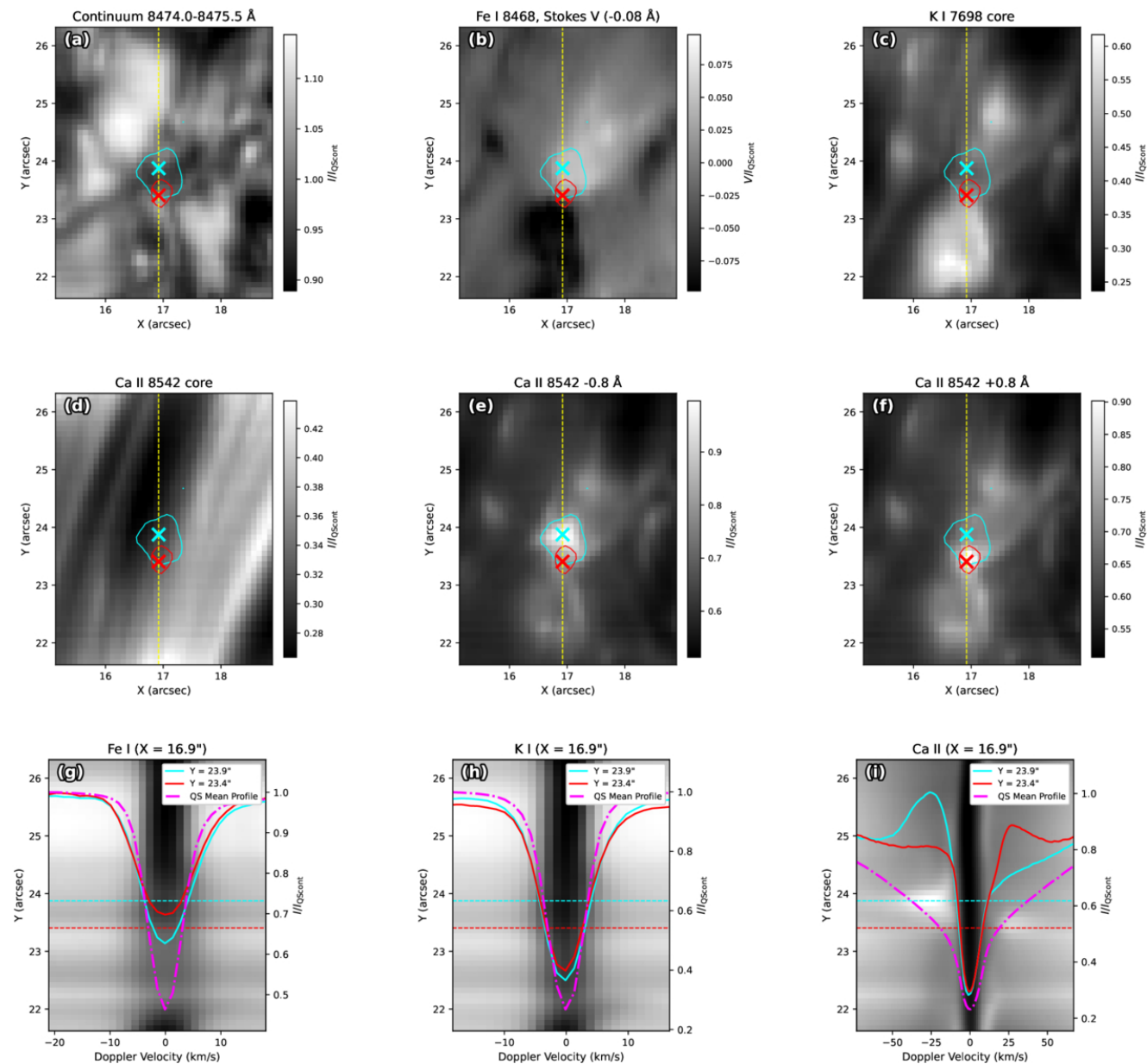
Figure 2. from Yusuke Kawabata et al 2026 Astrophys. J. Lett. 1007 doi:10.3847/2041-8213/ae91e0 https://dx.doi.org/10.3847/2041-8213/ae91e0 © 2026. The Author(s). Published by the American Astronomical Society.
