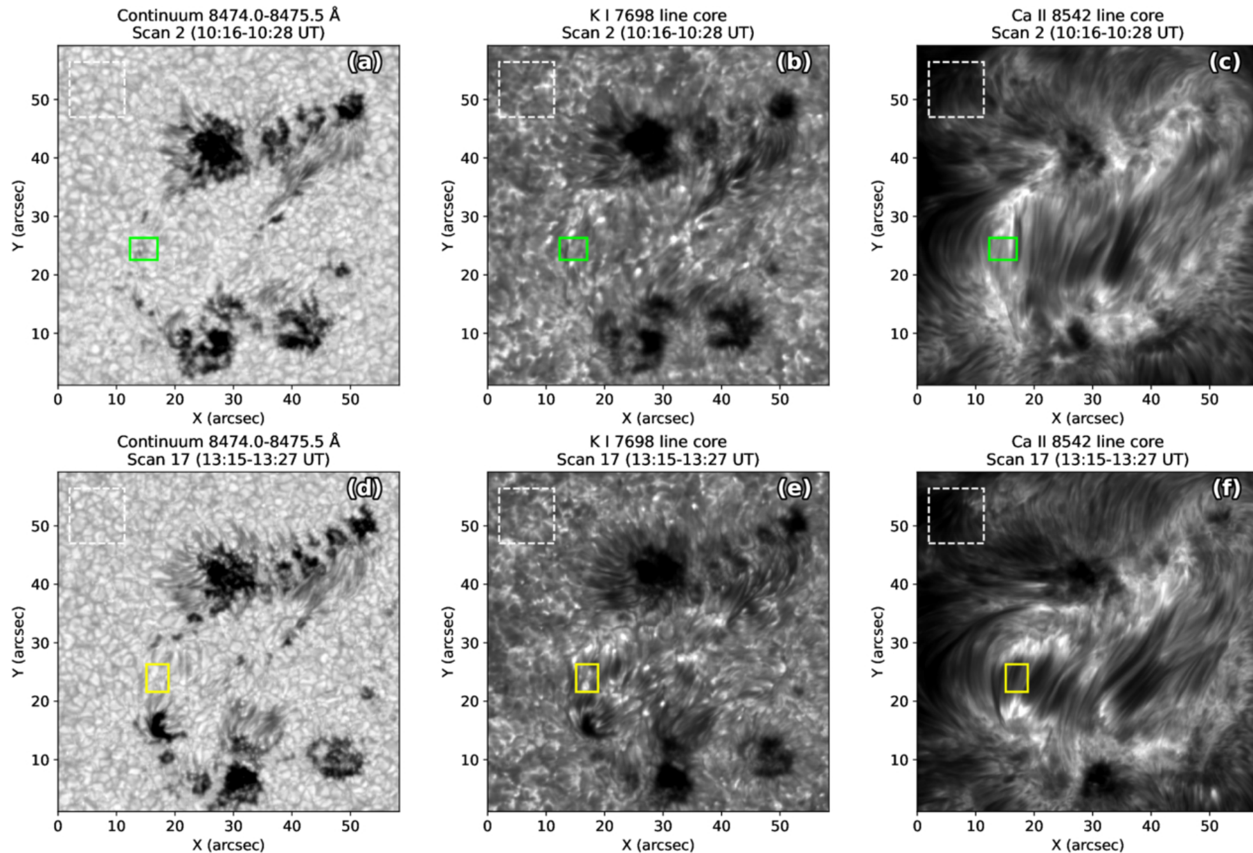
Figure 1. from Yusuke Kawabata et al 2026 Astrophys. J. Lett. 1007 doi:10.3847/2041-8213/ae91e0 https://dx.doi.org/10.3847/2041-8213/ae91e0 © 2026. The Author(s). Published by the American Astronomical Society.
