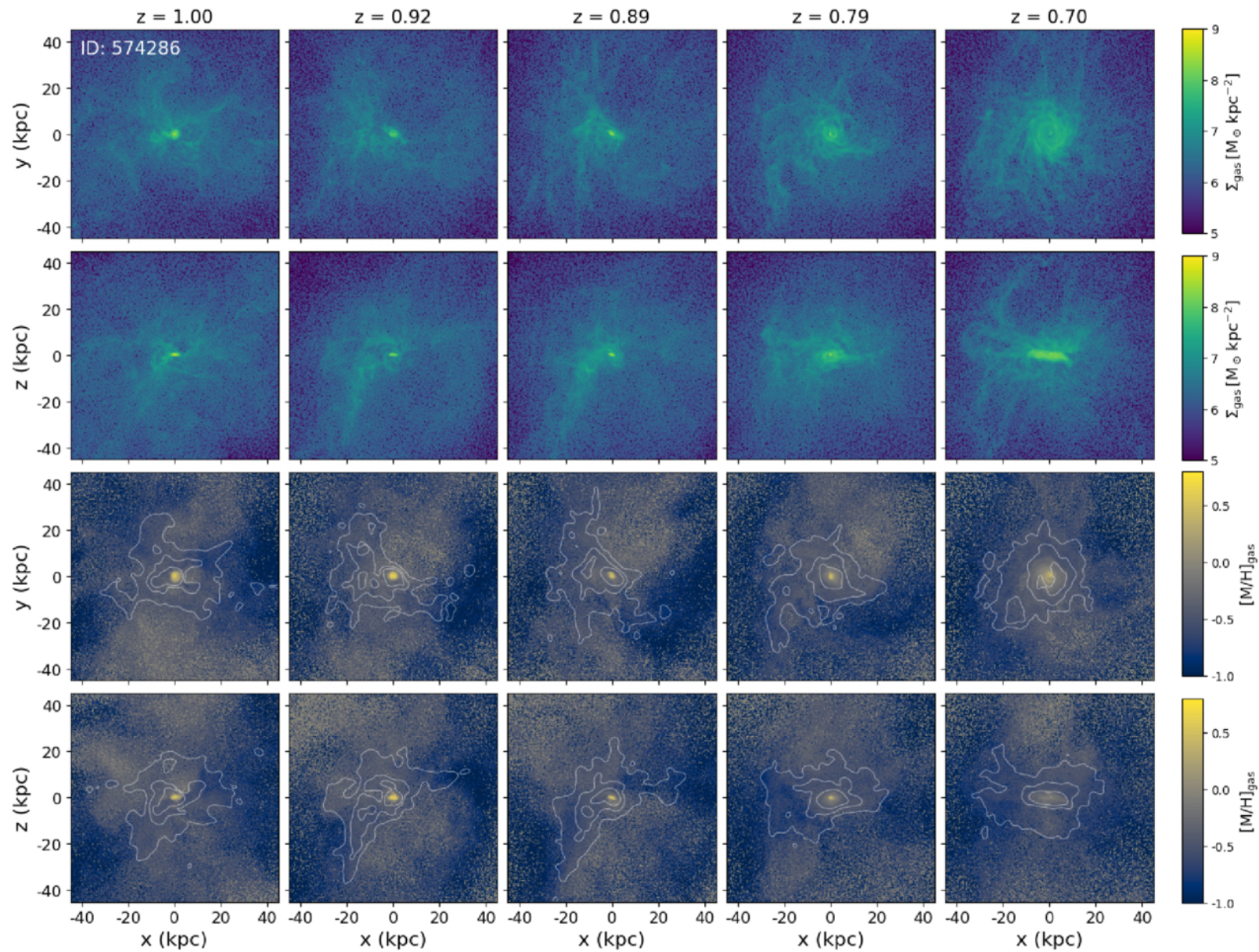
Figure 5. from Jianhui Lian et al 2026 Astrophys. J. Lett. 1007 doi:10.3847/2041-8213/ae915f https://dx.doi.org/10.3847/2041-8213/ae915f © 2026. The Author(s). Published by the American Astronomical Society.
