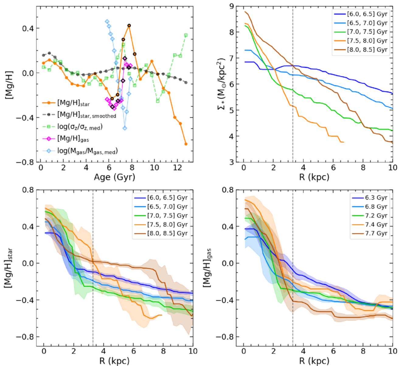
Figure 4. from Jianhui Lian et al 2026 Astrophys. J. Lett. 1007 doi:10.3847/2041-8213/ae915f https://dx.doi.org/10.3847/2041-8213/ae915f © 2026. The Author(s). Published by the American Astronomical Society.
