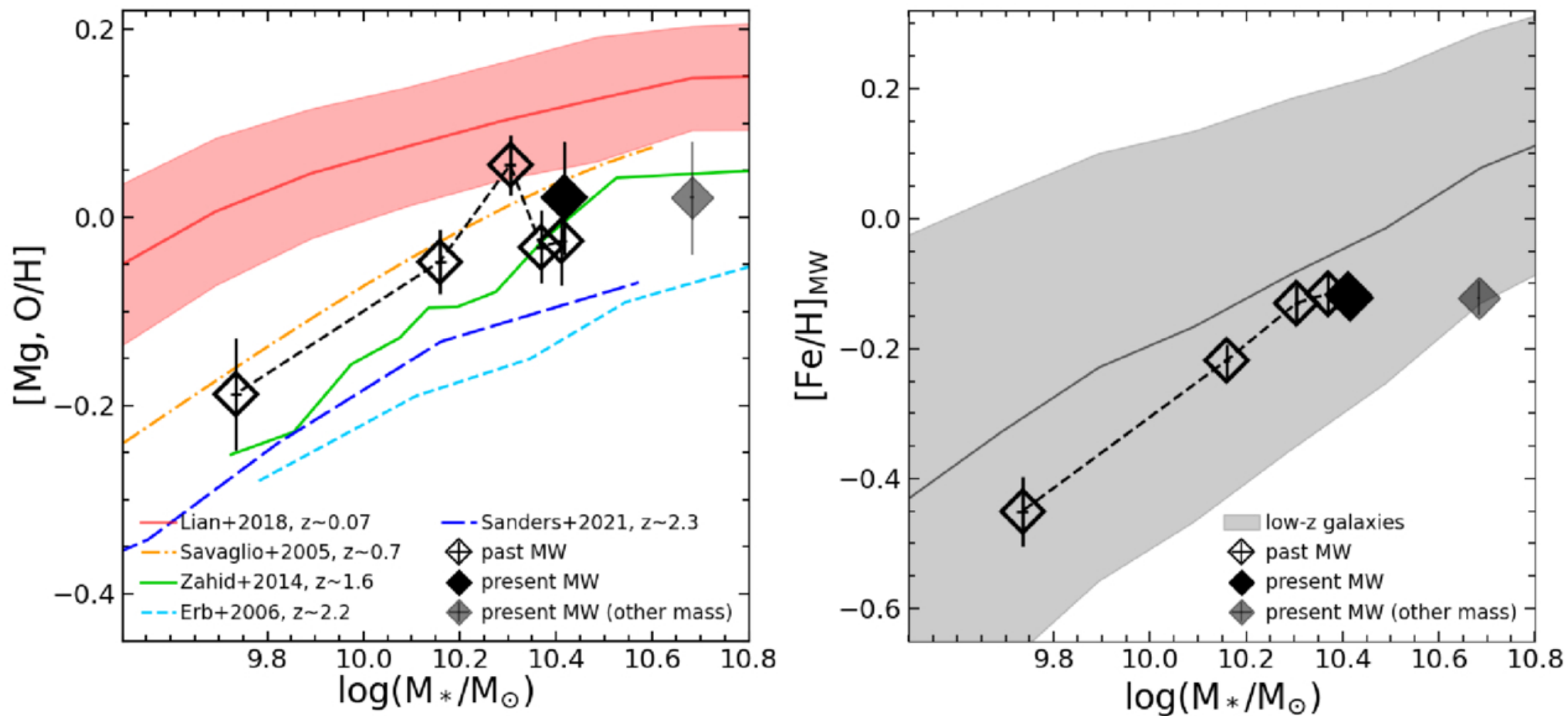
Figure 3. from Jianhui Lian et al 2026 Astrophys. J. Lett. 1007 doi:10.3847/2041-8213/ae915f https://dx.doi.org/10.3847/2041-8213/ae915f © 2026. The Author(s). Published by the American Astronomical Society.
