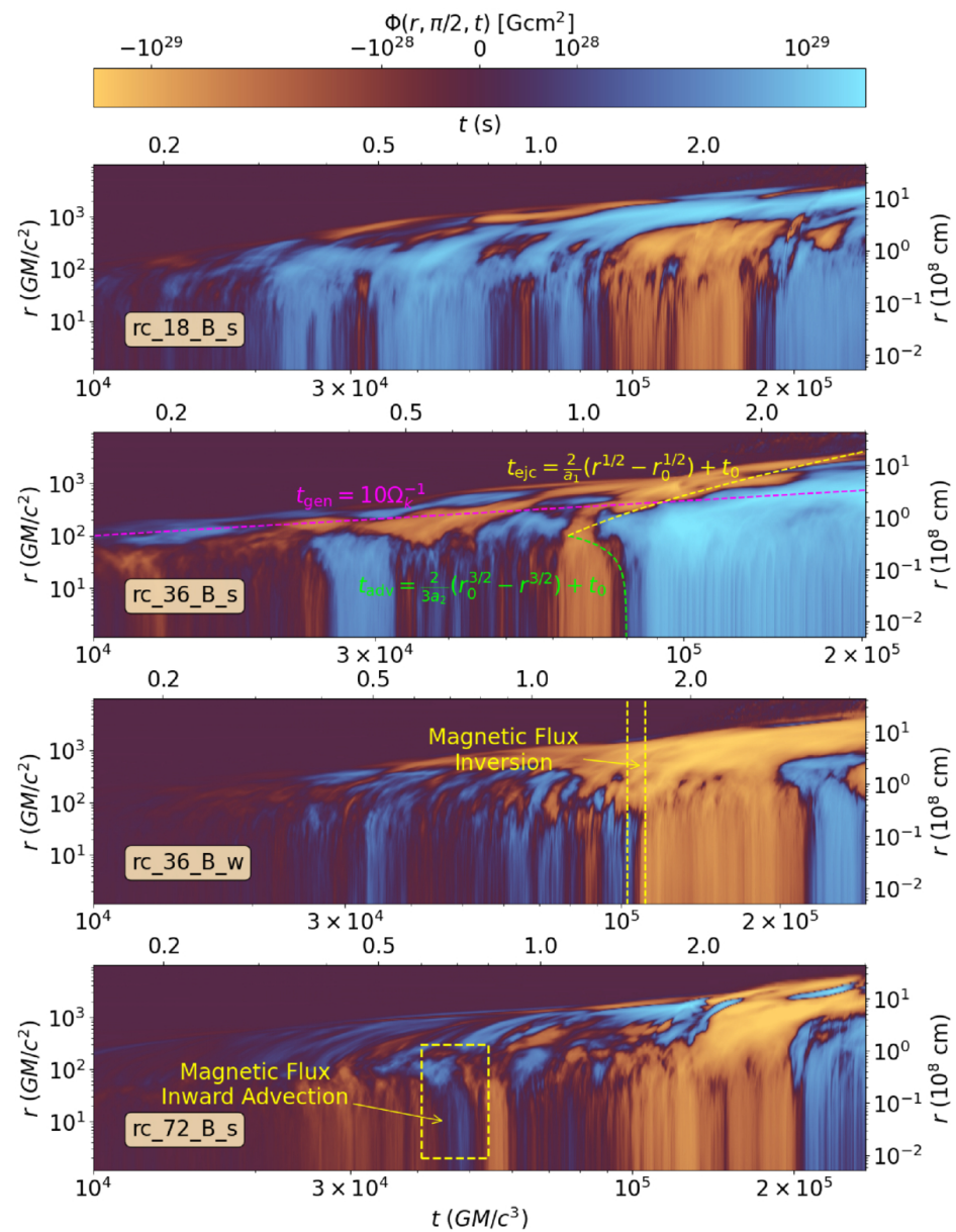
Figure 5. from Ho-Sang Chan et al 2026 Astrophys. J. Lett. 1007 doi:10.3847/2041-8213/ae9156 https://dx.doi.org/10.3847/2041-8213/ae9156 © 2026. The Author(s). Published by the American Astronomical Society.
