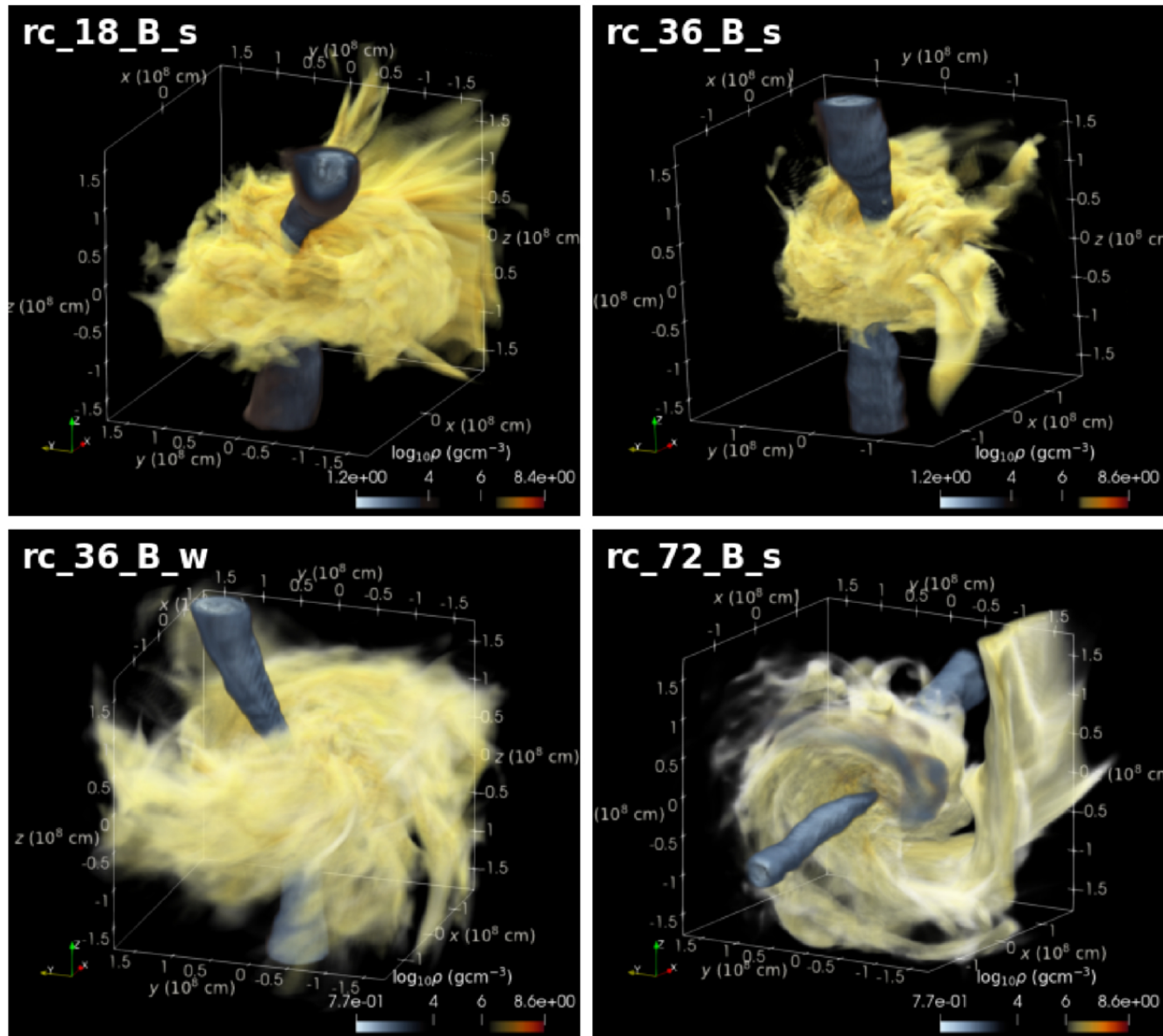
Figure 4. from Ho-Sang Chan et al 2026 Astrophys. J. Lett. 1007 doi:10.3847/2041-8213/ae9156 https://dx.doi.org/10.3847/2041-8213/ae9156 © 2026. The Author(s). Published by the American Astronomical Society.
