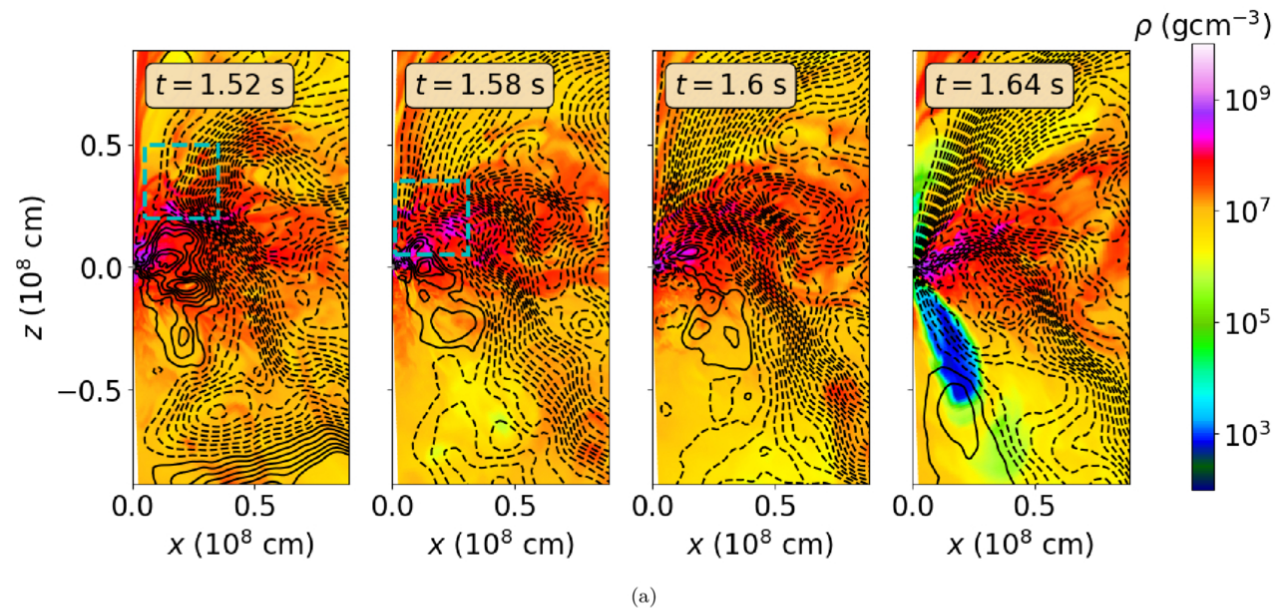
Figure 10. from Ho-Sang Chan et al 2026 Astrophys. J. Lett. 1007 doi:10.3847/2041-8213/ae9156 https://dx.doi.org/10.3847/2041-8213/ae9156 © 2026. The Author(s). Published by the American Astronomical Society.
