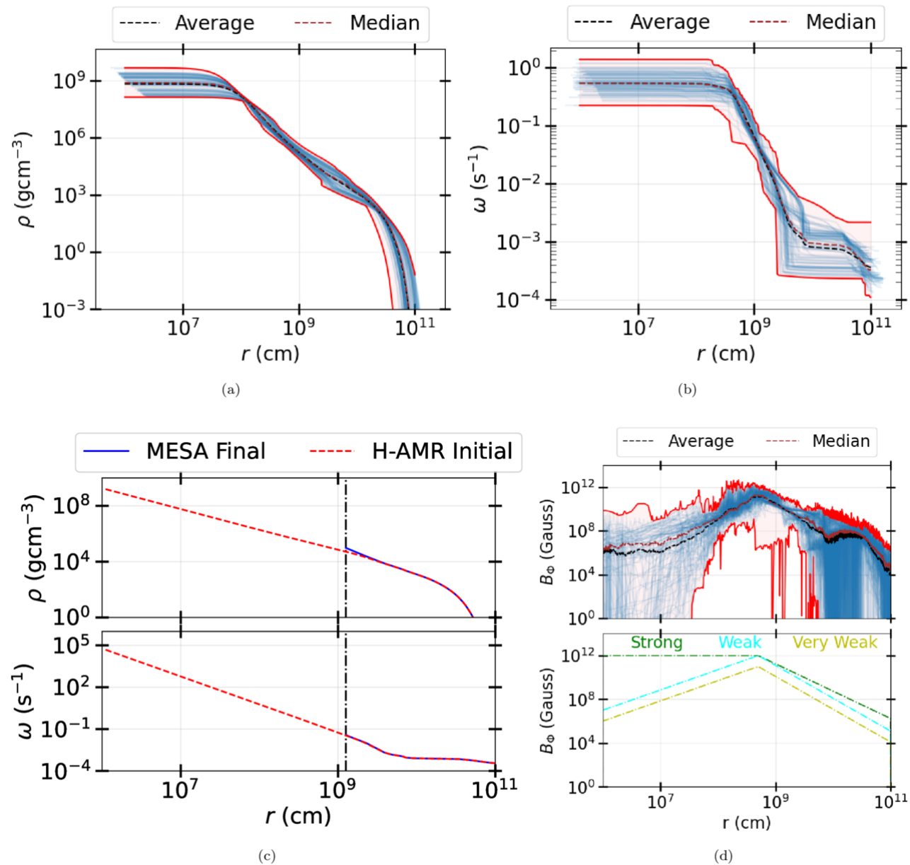
Figure 1. from Ho-Sang Chan et al 2026 Astrophys. J. Lett. 1007 doi:10.3847/2041-8213/ae9156 https://dx.doi.org/10.3847/2041-8213/ae9156 © 2026. The Author(s). Published by the American Astronomical Society.
