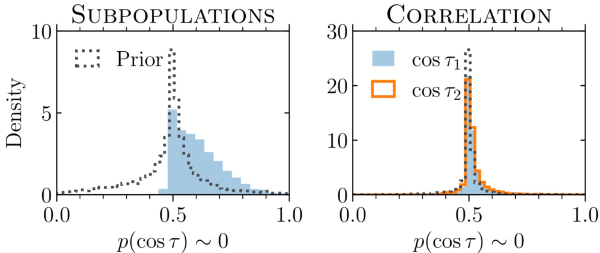
Figure E1. from Noah E. Wolfe et al 2026 Astrophys. J. Lett. 1007 doi:10.3847/2041-8213/ae90ae https://dx.doi.org/10.3847/2041-8213/ae90ae © 2026. The Author(s). Published by the American Astronomical Society.
