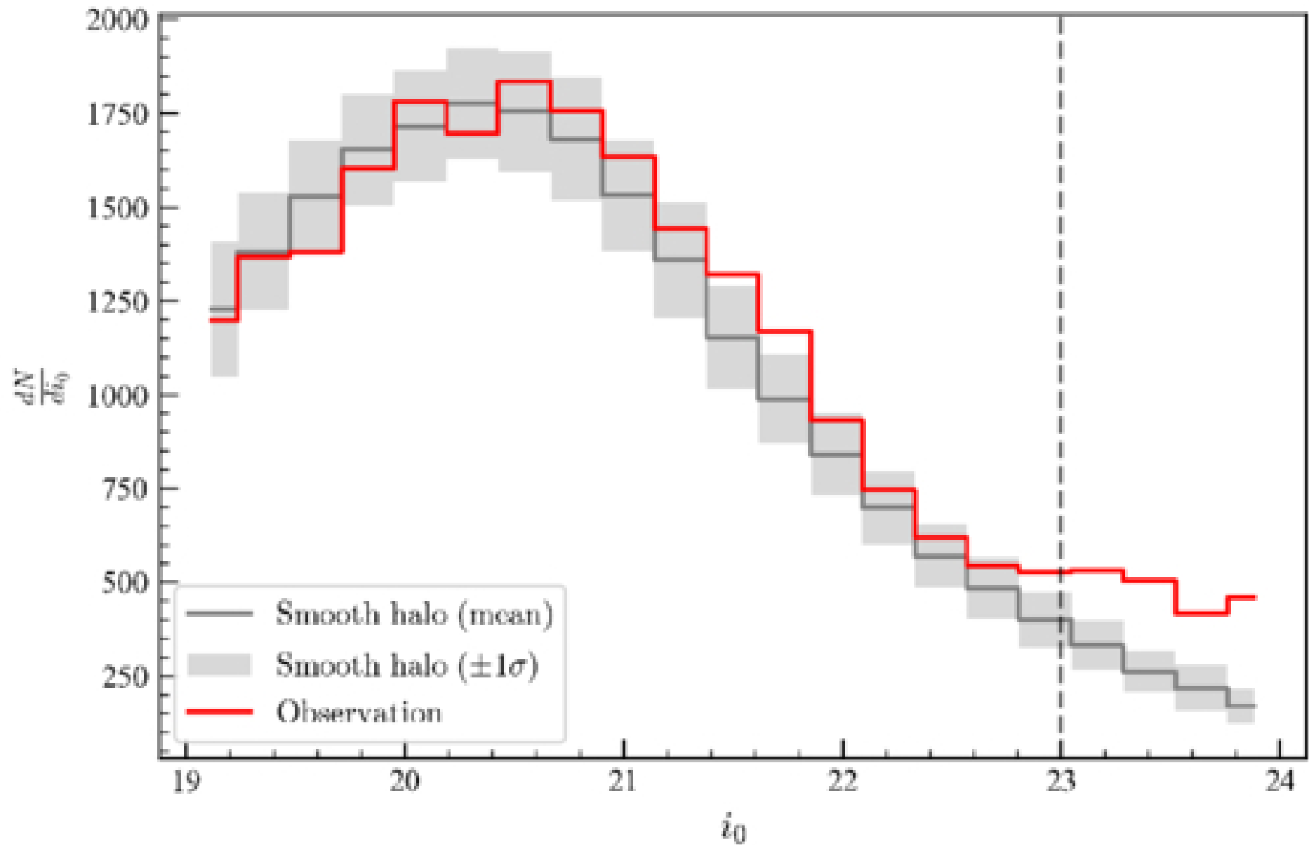
Figure 4. from Yoshihisa Suzuki et al 2026 Astrophys. J. Lett. 1007 doi:10.3847/2041-8213/ae909f https://dx.doi.org/10.3847/2041-8213/ae909f © 2026. The Author(s). Published by the American Astronomical Society.
