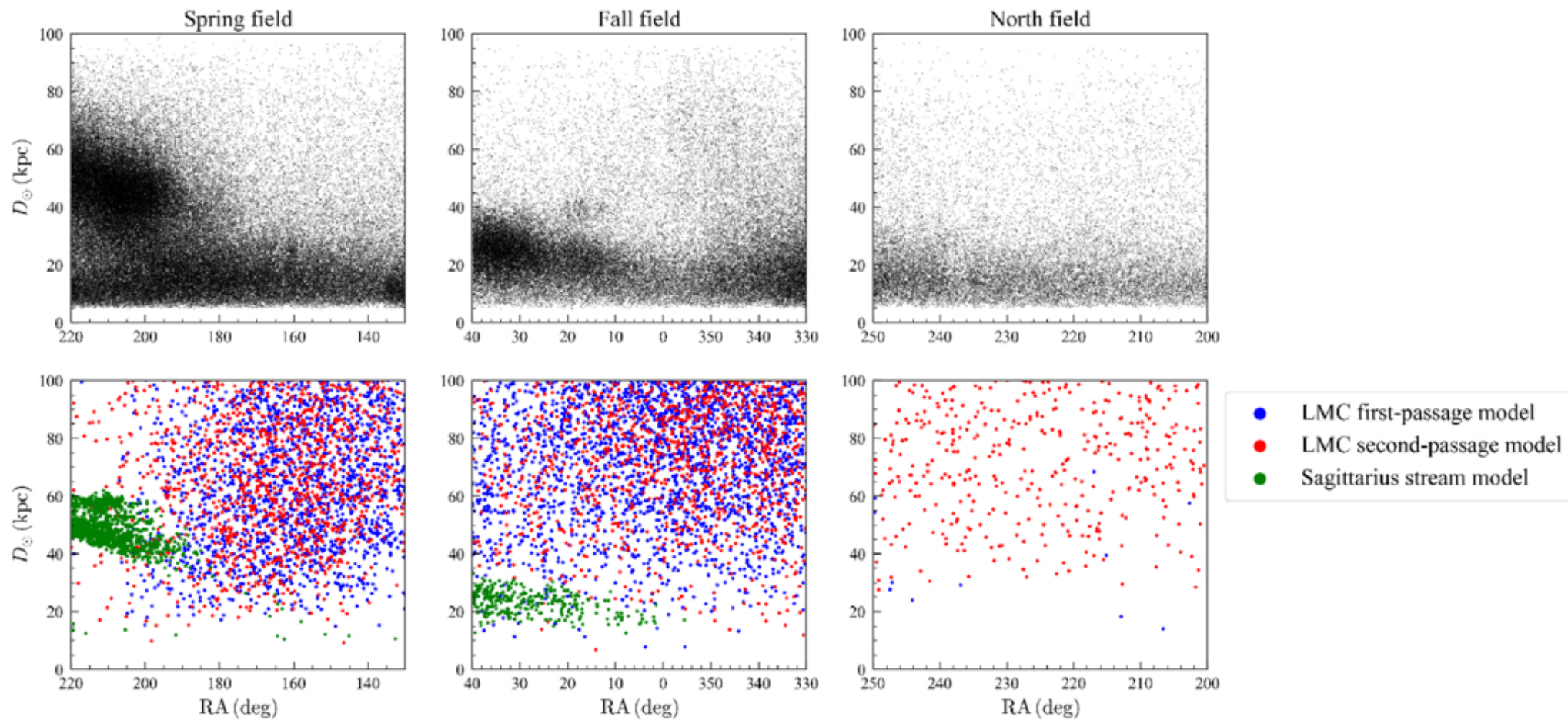
Figure 3. from Yoshihisa Suzuki et al 2026 Astrophys. J. Lett. 1007 doi:10.3847/2041-8213/ae909f https://dx.doi.org/10.3847/2041-8213/ae909f © 2026. The Author(s). Published by the American Astronomical Society.
