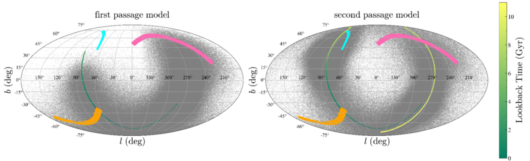
Figure 1. from Yoshihisa Suzuki et al 2026 Astrophys. J. Lett. 1007 doi:10.3847/2041-8213/ae909f https://dx.doi.org/10.3847/2041-8213/ae909f © 2026. The Author(s). Published by the American Astronomical Society.
