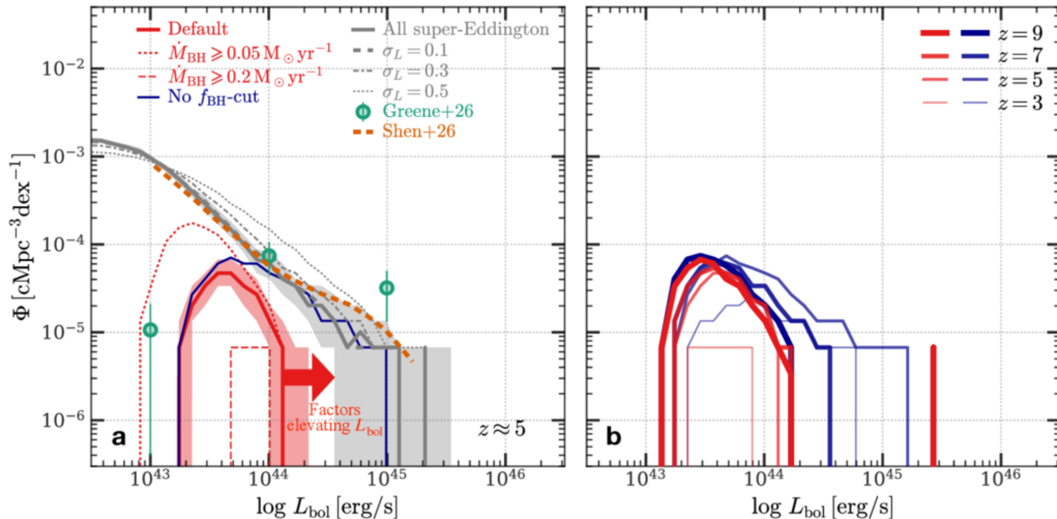
Figure 4. from Yangyao Chen and Houjun Mo 2026 Astrophys. J. Lett. 1007 doi:10.3847/2041-8213/ae909e https://dx.doi.org/10.3847/2041-8213/ae909e © 2026. The Author(s). Published by the American Astronomical Society.
