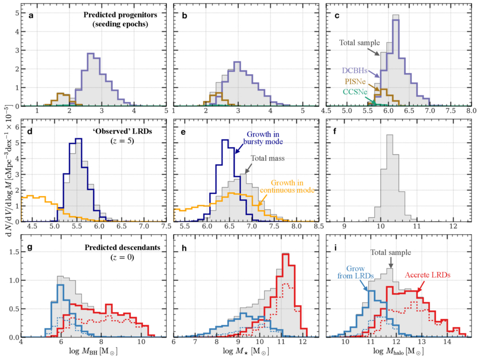
Figure 3. from Yangyao Chen and Houjun Mo 2026 Astrophys. J. Lett. 1007 doi:10.3847/2041-8213/ae909e https://dx.doi.org/10.3847/2041-8213/ae909e © 2026. The Author(s). Published by the American Astronomical Society.
