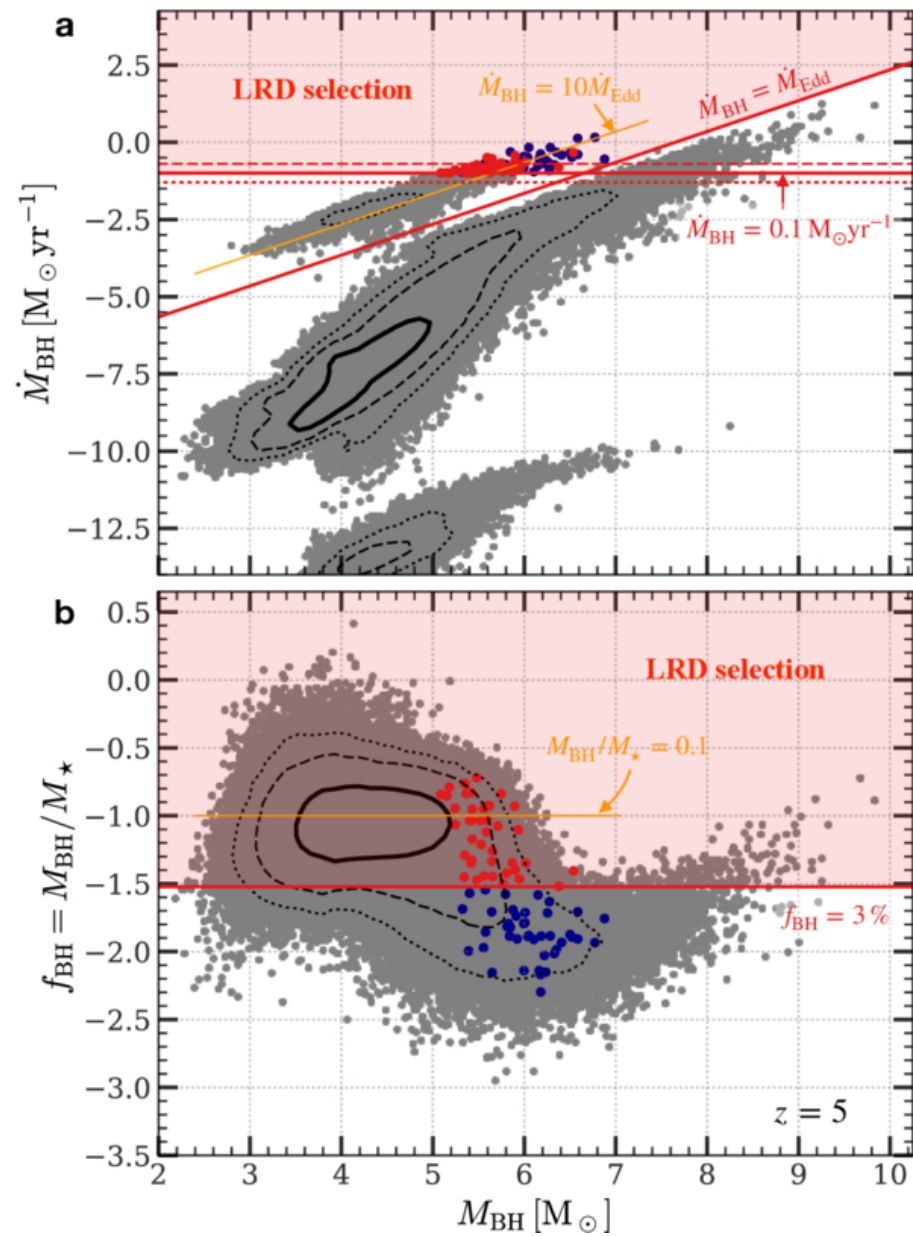
Figure 1. from Yangyao Chen and Houjun Mo 2026 Astrophys. J. Lett. 1007 doi:10.3847/2041-8213/ae909e https://dx.doi.org/10.3847/2041-8213/ae909e © 2026. The Author(s). Published by the American Astronomical Society.
