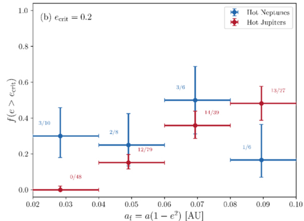
Figure 6. from Cristobal Petrovich and Hareesh Gautham Bhaskar 2026 Astrophys. J. Lett. 1007 doi:10.3847/2041-8213/ae909d https://dx.doi.org/10.3847/2041-8213/ae909d © 2026. The Author(s). Published by the American Astronomical Society.
