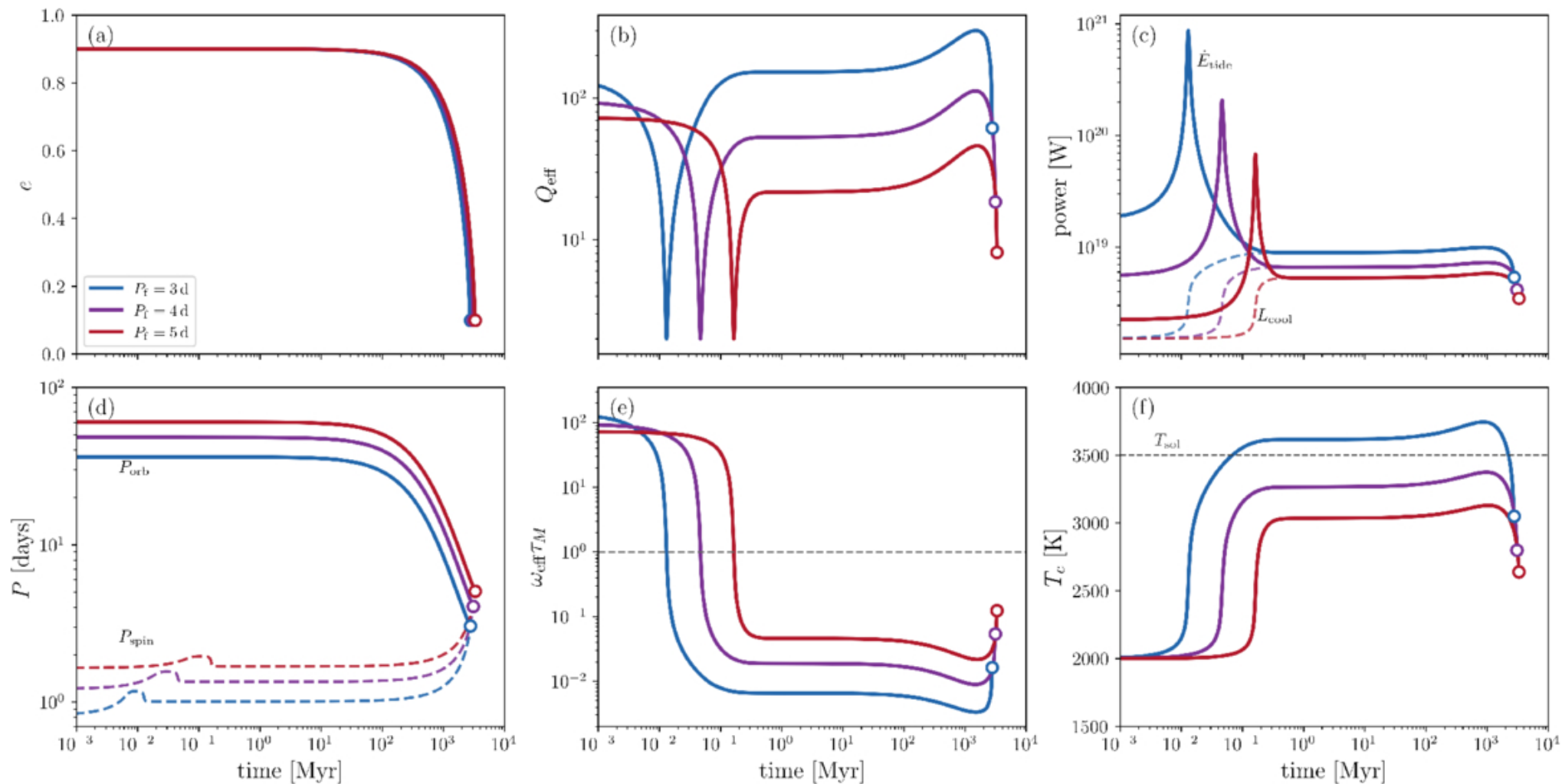
Figure 4. from Cristobal Petrovich and Hareesh Gautham Bhaskar 2026 Astrophys. J. Lett. 1007 doi:10.3847/2041-8213/ae909d https://dx.doi.org/10.3847/2041-8213/ae909d © 2026. The Author(s). Published by the American Astronomical Society.
