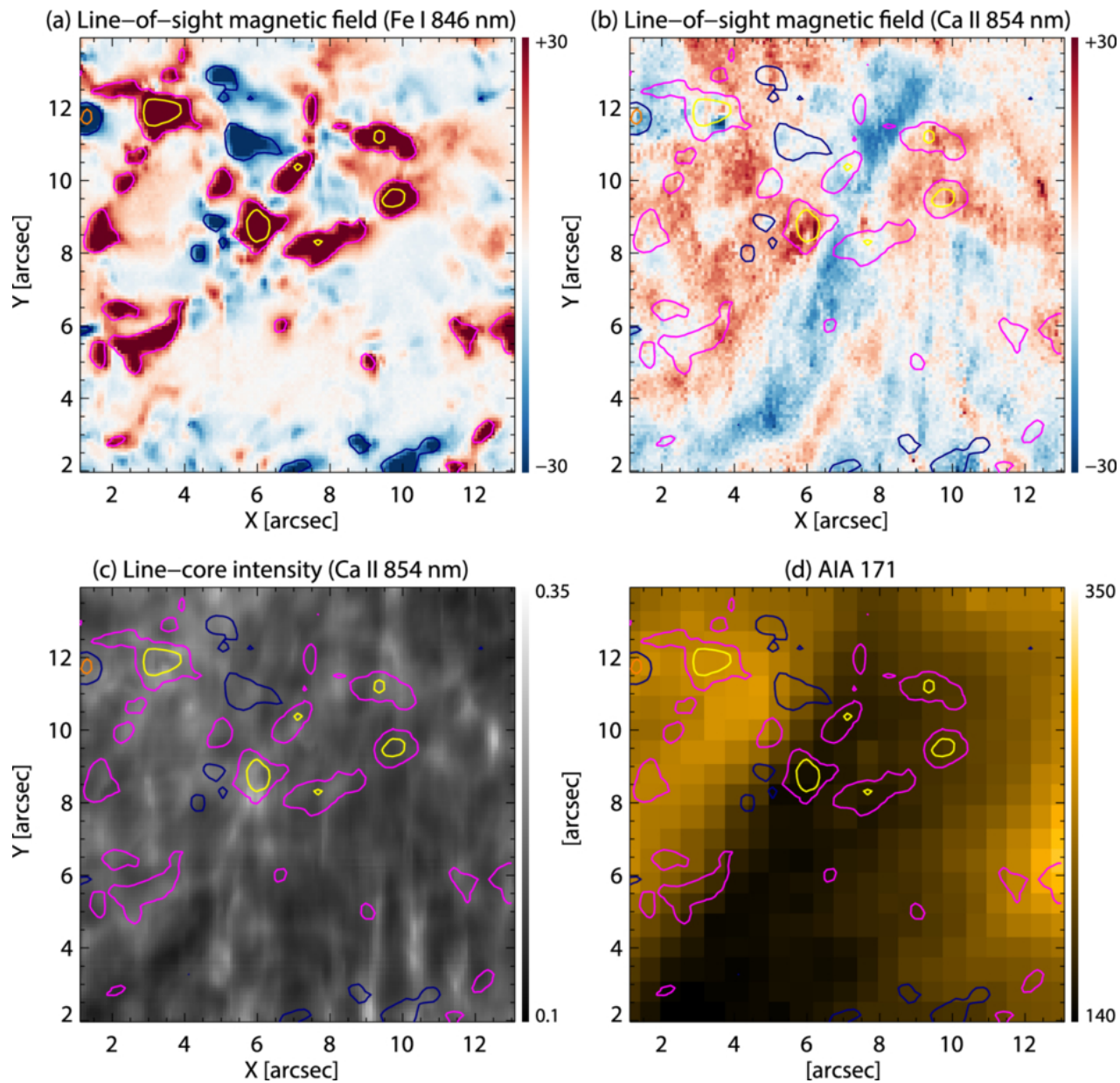
Figure 5. from Masahito Kubo et al 2026 Astrophys. J. Lett. 1008 doi:10.3847/2041-8213/ae909b https://dx.doi.org/10.3847/2041-8213/ae909b © 2026. The Author(s). Published by the American Astronomical Society.
