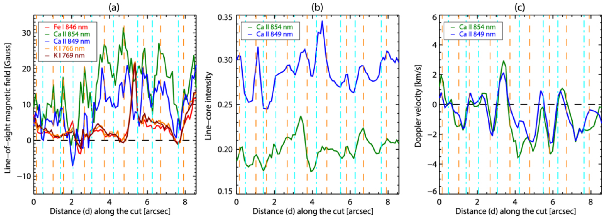
Figure 4. from Masahito Kubo et al 2026 Astrophys. J. Lett. 1008 doi:10.3847/2041-8213/ae909b https://dx.doi.org/10.3847/2041-8213/ae909b © 2026. The Author(s). Published by the American Astronomical Society.
