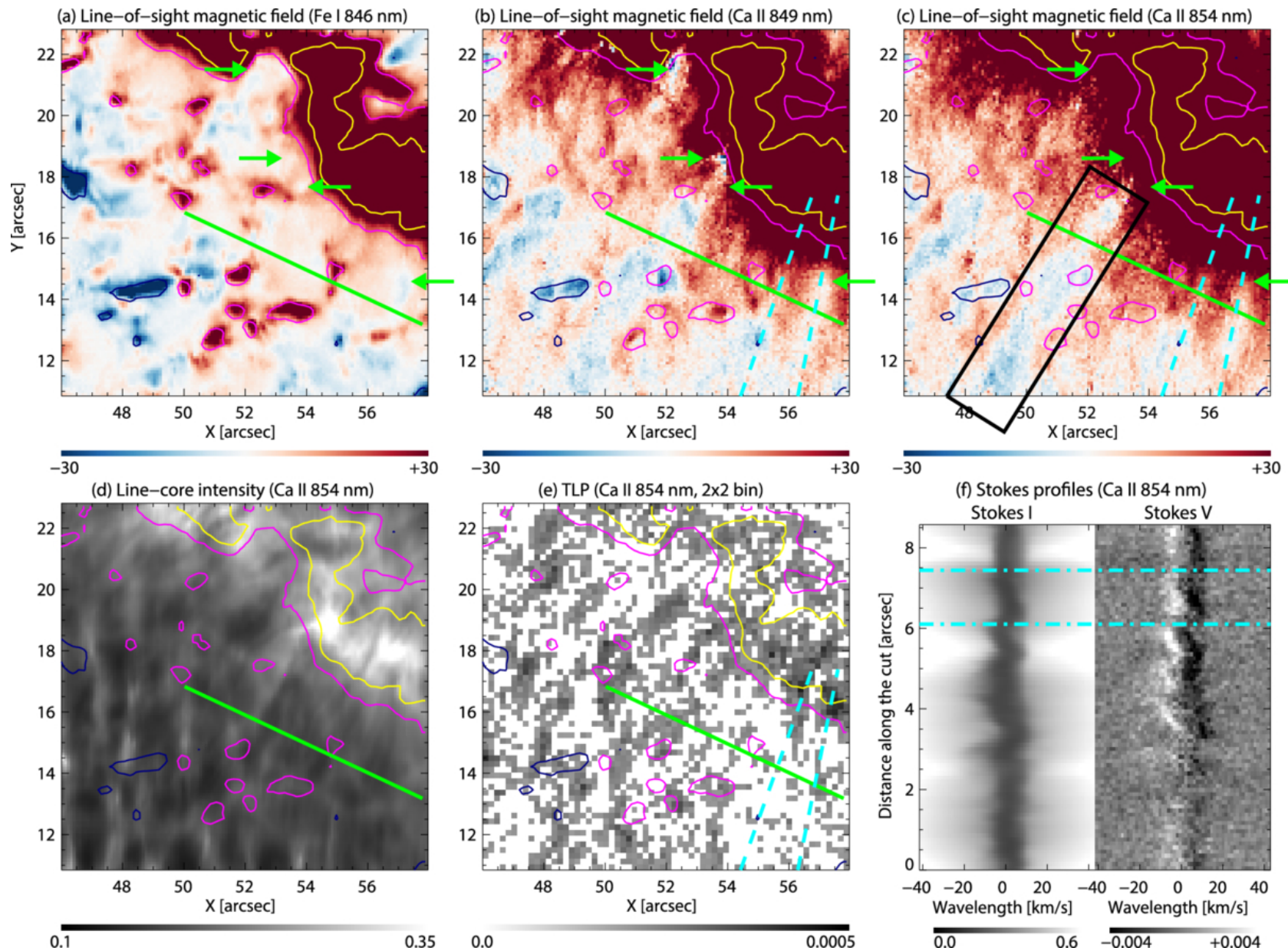
Figure 3. from Masahito Kubo et al 2026 Astrophys. J. Lett. 1008 doi:10.3847/2041-8213/ae909b https://dx.doi.org/10.3847/2041-8213/ae909b © 2026. The Author(s). Published by the American Astronomical Society.
