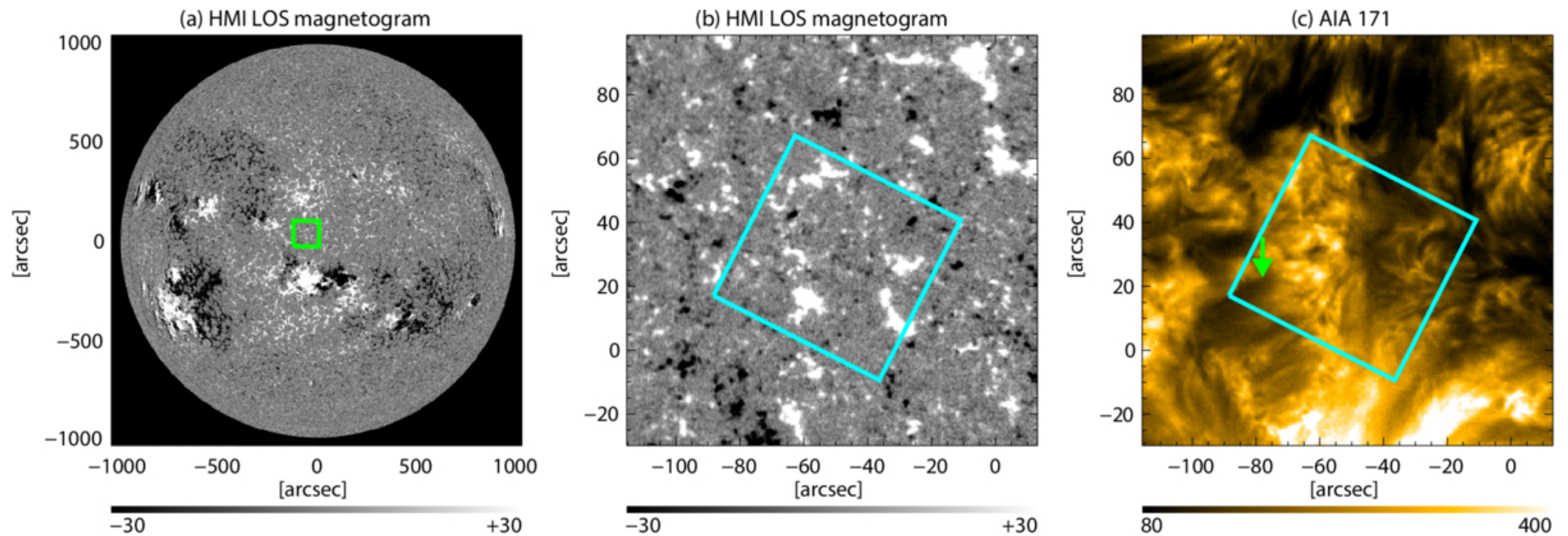
Figure 1. from Masahito Kubo et al 2026 Astrophys. J. Lett. 1008 doi:10.3847/2041-8213/ae909b https://dx.doi.org/10.3847/2041-8213/ae909b © 2026. The Author(s). Published by the American Astronomical Society.
