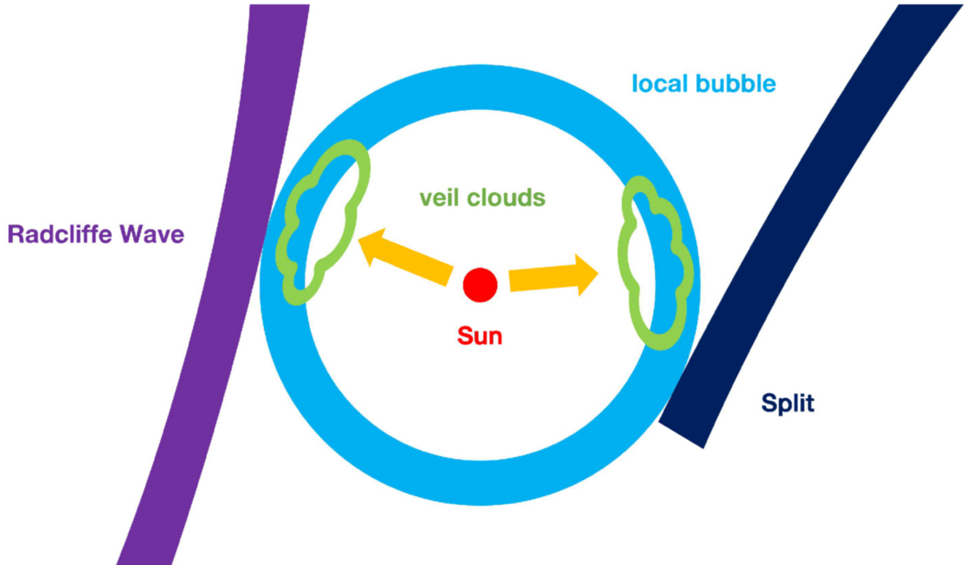
Figure 6. from Ruilin Xia et al 2026 Astrophys. J. Lett. 1007 doi:10.3847/2041-8213/ae9091 https://dx.doi.org/10.3847/2041-8213/ae9091 © 2026. The Author(s). Published by the American Astronomical Society.
