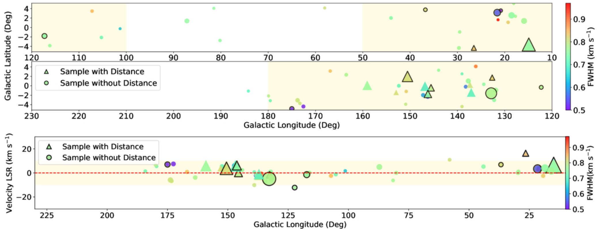
Figure 4. from Ruilin Xia et al 2026 Astrophys. J. Lett. 1007 doi:10.3847/2041-8213/ae9091 https://dx.doi.org/10.3847/2041-8213/ae9091 © 2026. The Author(s). Published by the American Astronomical Society.
