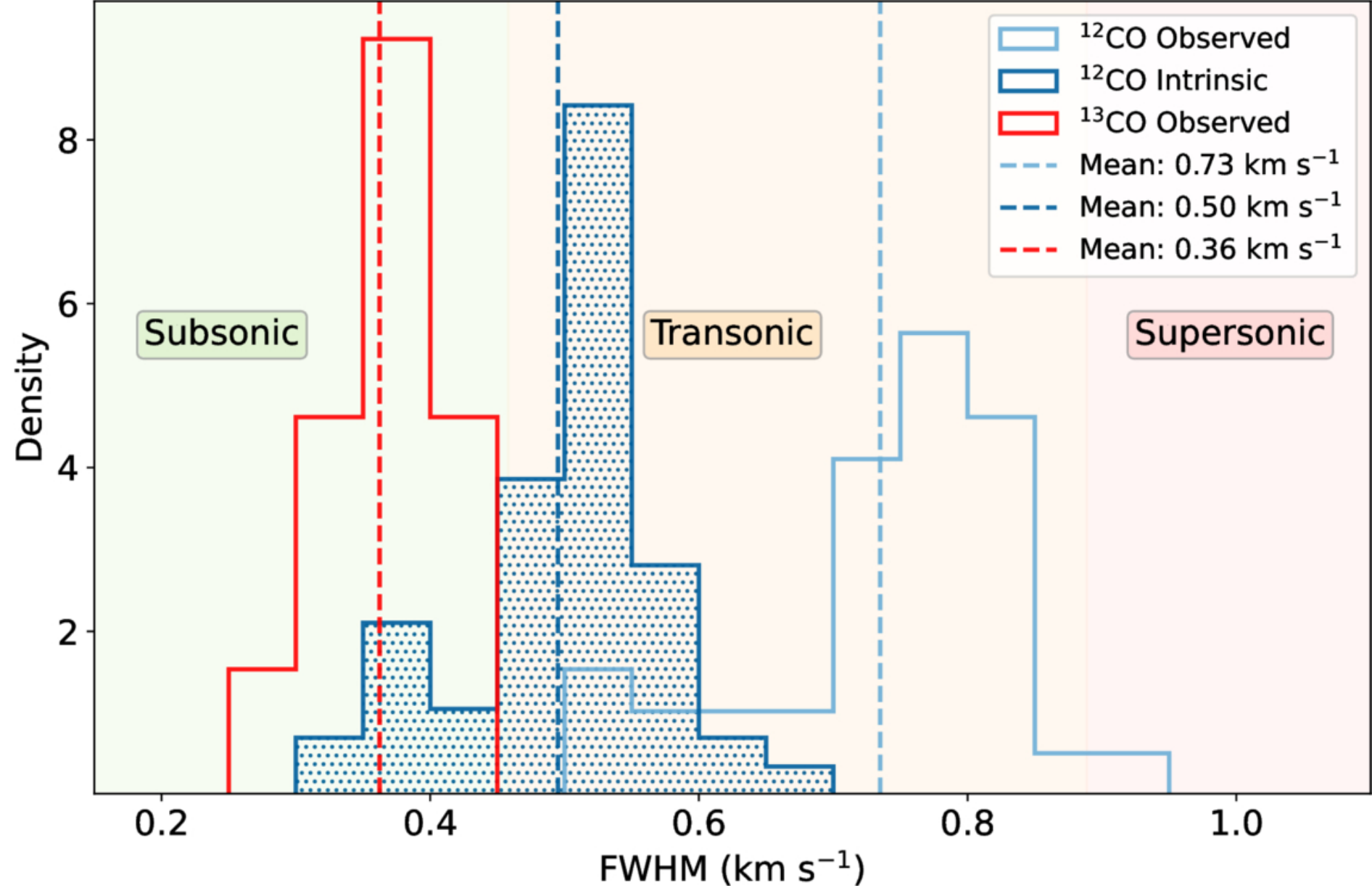
Figure 3. from Ruilin Xia et al 2026 Astrophys. J. Lett. 1007 doi:10.3847/2041-8213/ae9091 https://dx.doi.org/10.3847/2041-8213/ae9091 © 2026. The Author(s). Published by the American Astronomical Society.
