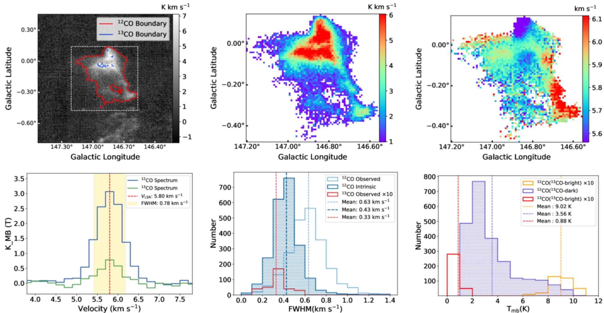
Figure 2. from Ruilin Xia et al 2026 Astrophys. J. Lett. 1007 doi:10.3847/2041-8213/ae9091 https://dx.doi.org/10.3847/2041-8213/ae9091 © 2026. The Author(s). Published by the American Astronomical Society.
