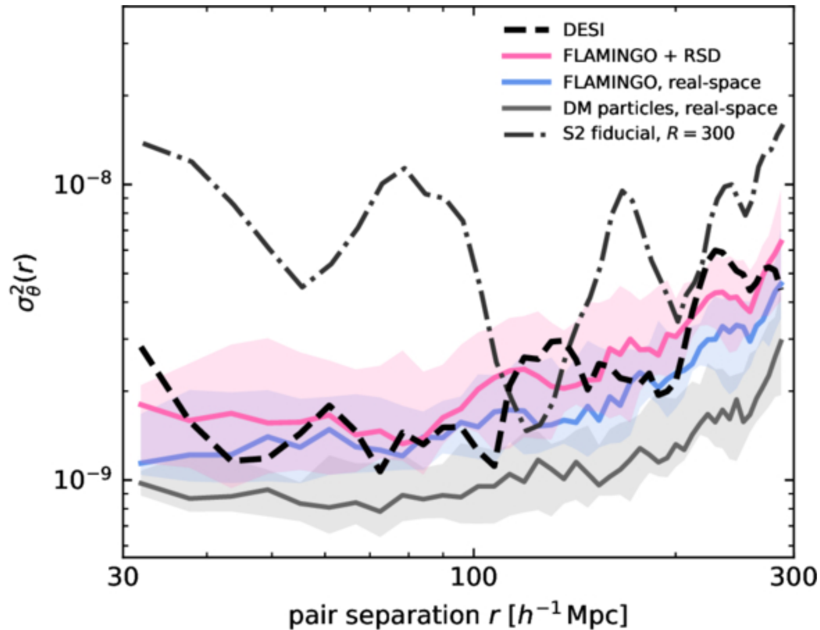
Figure 9. from Till Sawala 2026 Astrophys. J. Lett. 1007 doi:10.3847/2041-8213/ae908f https://dx.doi.org/10.3847/2041-8213/ae908f © 2026. The Author(s). Published by the American Astronomical Society.
