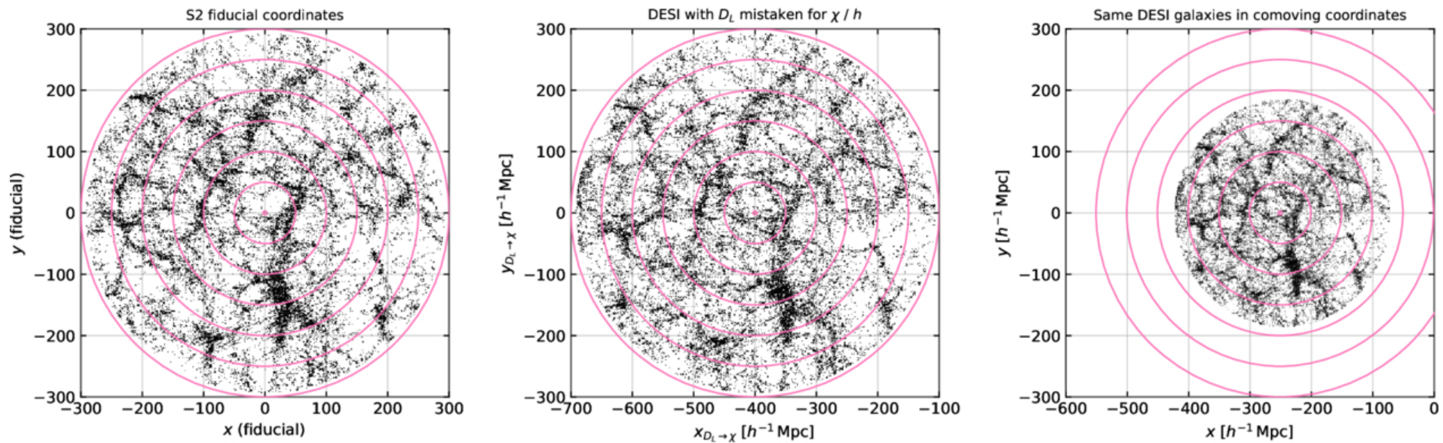
Figure 5. from Till Sawala 2026 Astrophys. J. Lett. 1007 doi:10.3847/2041-8213/ae908f https://dx.doi.org/10.3847/2041-8213/ae908f © 2026. The Author(s). Published by the American Astronomical Society.
