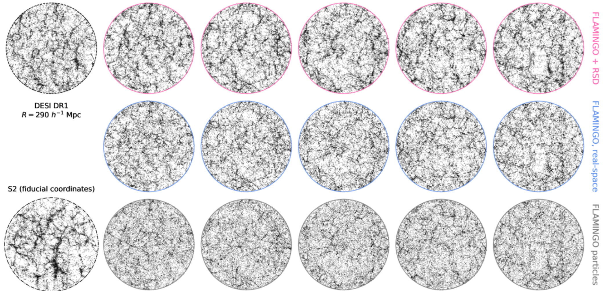
Figure 2. from Till Sawala 2026 Astrophys. J. Lett. 1007 doi:10.3847/2041-8213/ae908f https://dx.doi.org/10.3847/2041-8213/ae908f © 2026. The Author(s). Published by the American Astronomical Society.
