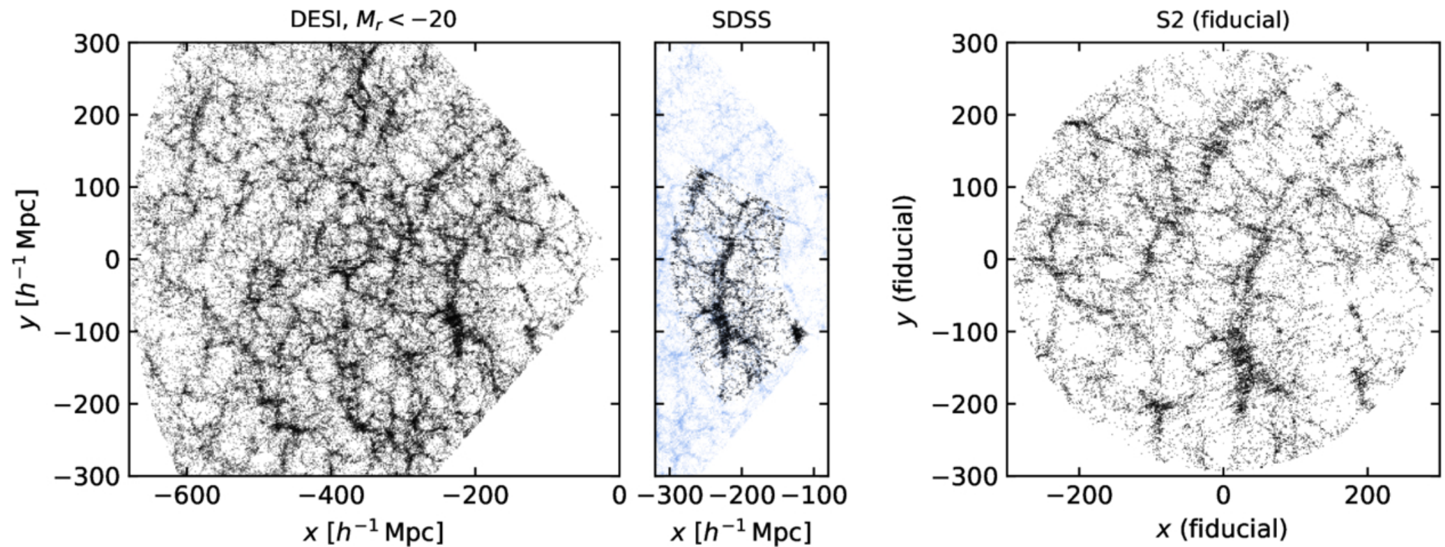
Figure 1. from Till Sawala 2026 Astrophys. J. Lett. 1007 doi:10.3847/2041-8213/ae908f https://dx.doi.org/10.3847/2041-8213/ae908f © 2026. The Author(s). Published by the American Astronomical Society.
