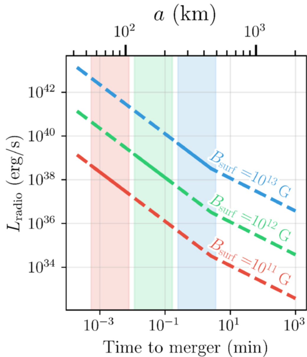
Figure 7. from Jasmine Parsons et al 2026 Astrophys. J. Lett. 1007 doi:10.3847/2041-8213/ae9088 https://dx.doi.org/10.3847/2041-8213/ae9088 © 2026. The Author(s). Published by the American Astronomical Society.
