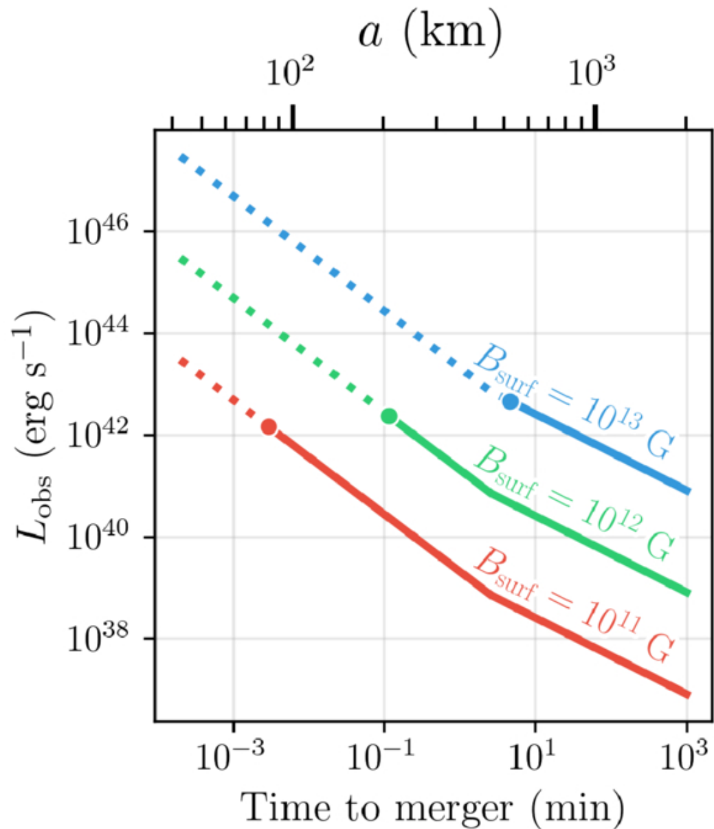
Figure 6. from Jasmine Parsons et al 2026 Astrophys. J. Lett. 1007 doi:10.3847/2041-8213/ae9088 https://dx.doi.org/10.3847/2041-8213/ae9088 © 2026. The Author(s). Published by the American Astronomical Society.
