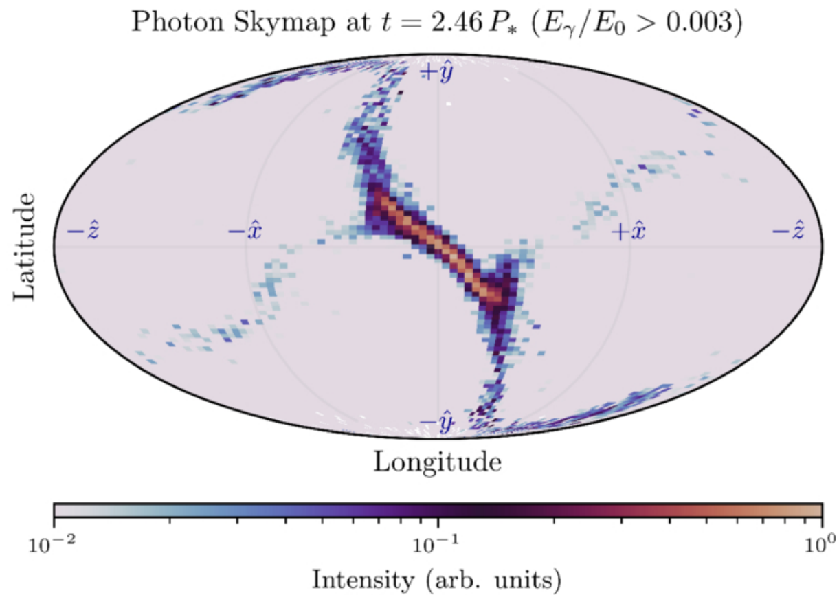
Figure 5. from Jasmine Parsons et al 2026 Astrophys. J. Lett. 1007 doi:10.3847/2041-8213/ae9088 https://dx.doi.org/10.3847/2041-8213/ae9088 © 2026. The Author(s). Published by the American Astronomical Society.
