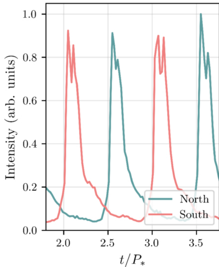
Figure 5. from Jasmine Parsons et al 2026 Astrophys. J. Lett. 1007 doi:10.3847/2041-8213/ae9088 https://dx.doi.org/10.3847/2041-8213/ae9088 © 2026. The Author(s). Published by the American Astronomical Society.
