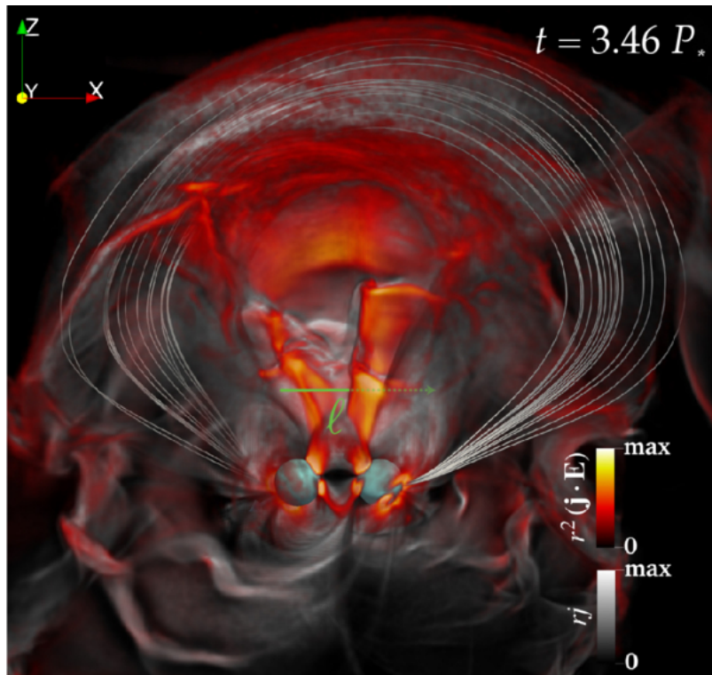
Figure 3. from Jasmine Parsons et al 2026 Astrophys. J. Lett. 1007 doi:10.3847/2041-8213/ae9088 https://dx.doi.org/10.3847/2041-8213/ae9088 © 2026. The Author(s). Published by the American Astronomical Society.
