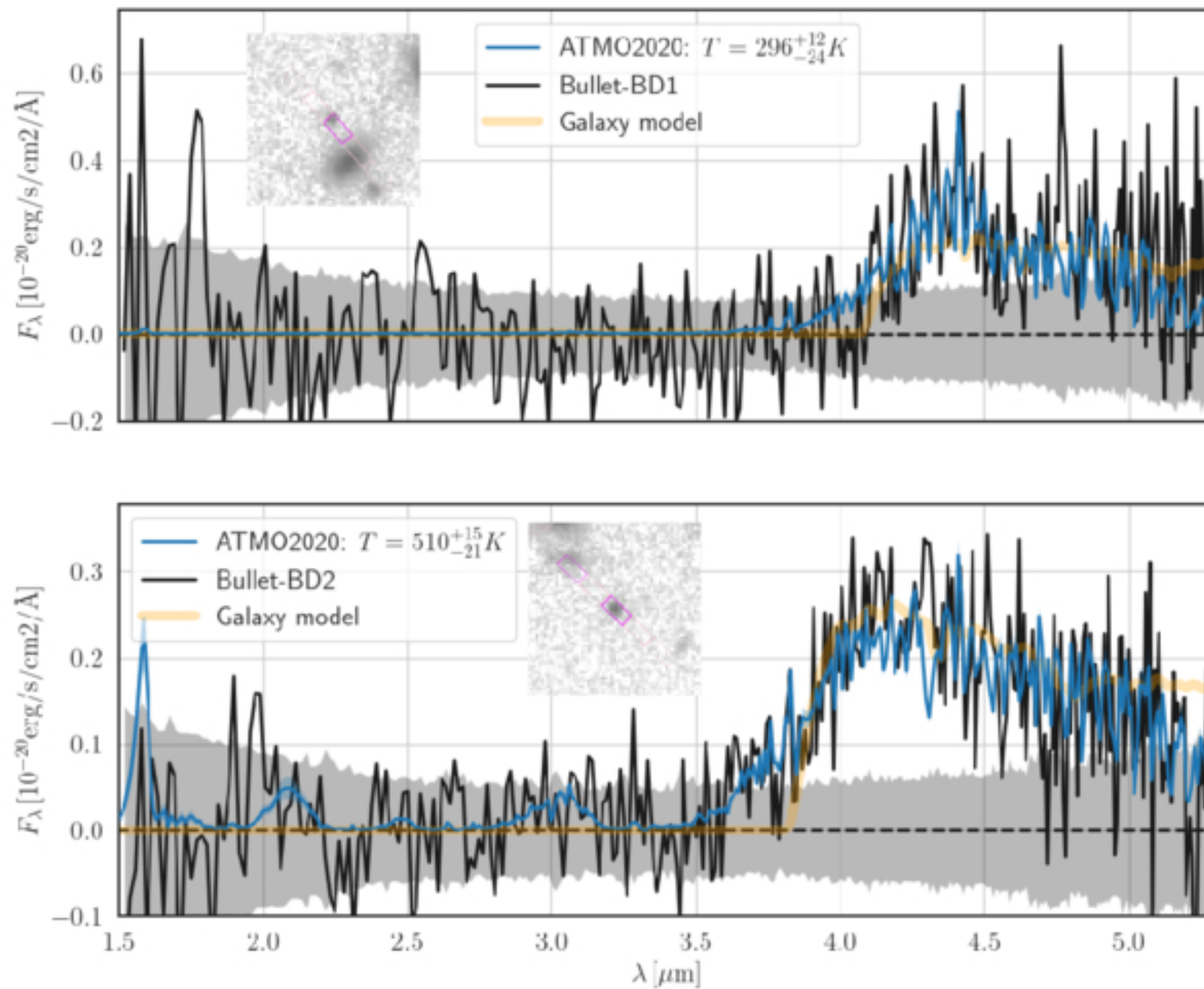
Figure 2. from Maruša Bradac et al 2026 Astrophys. J. Lett. 1010 doi:10.3847/2041-8213/ae9085 https://dx.doi.org/10.3847/2041-8213/ae9085 © 2026. The Author(s). Published by the American Astronomical Society.
