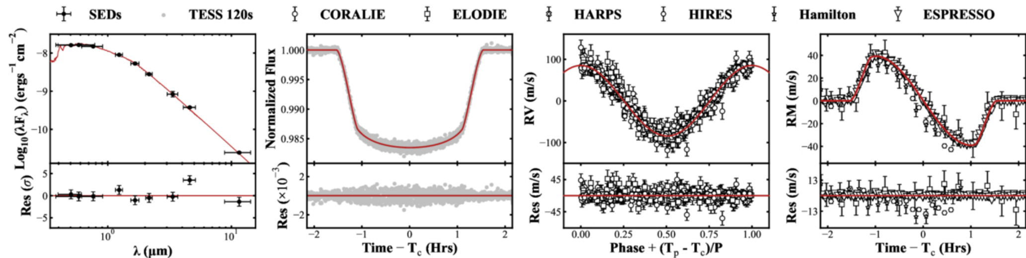
Figure 1. from Xian-Yu Wang et al 2026 Astrophys. J. Lett. 1008 doi:10.3847/2041-8213/ae907d https://dx.doi.org/10.3847/2041-8213/ae907d © 2026. The Author(s). Published by the American Astronomical Society.
