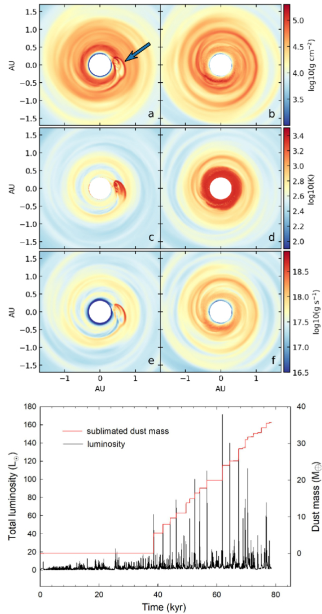
Figure 5. from Eduard I. Vorobyov et al 2026 Astrophys. J. Lett. 1007 doi:10.3847/2041-8213/ae907c https://dx.doi.org/10.3847/2041-8213/ae907c © 2026. The Author(s). Published by the American Astronomical Society.
