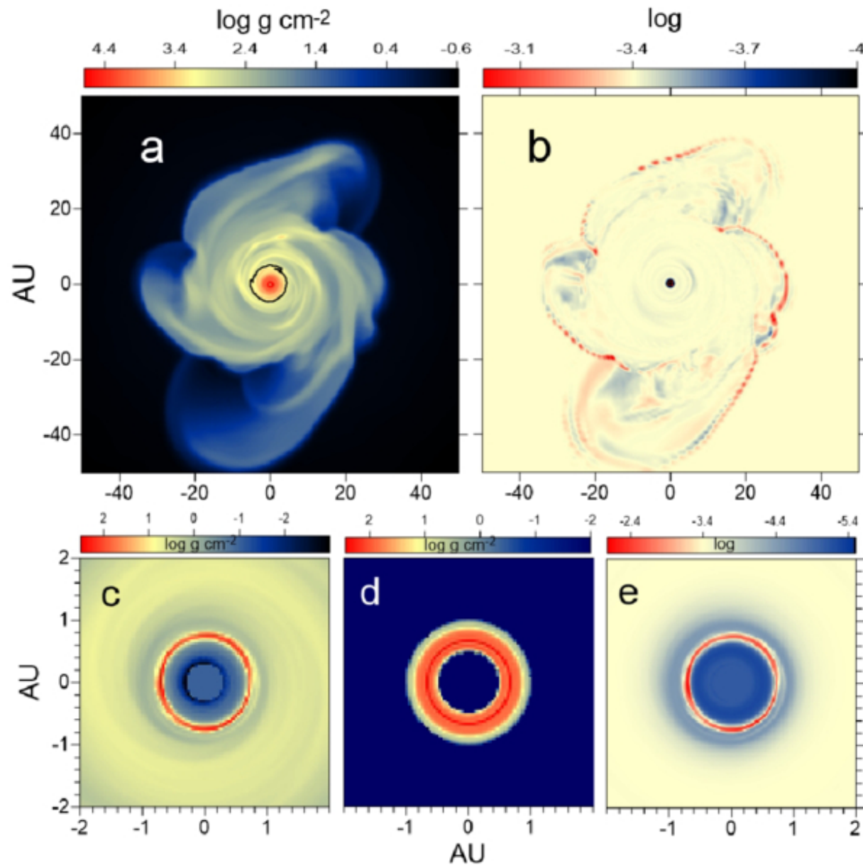
Figure 4. from Eduard I. Vorobyov et al 2026 Astrophys. J. Lett. 1007 doi:10.3847/2041-8213/ae907c https://dx.doi.org/10.3847/2041-8213/ae907c © 2026. The Author(s). Published by the American Astronomical Society.
