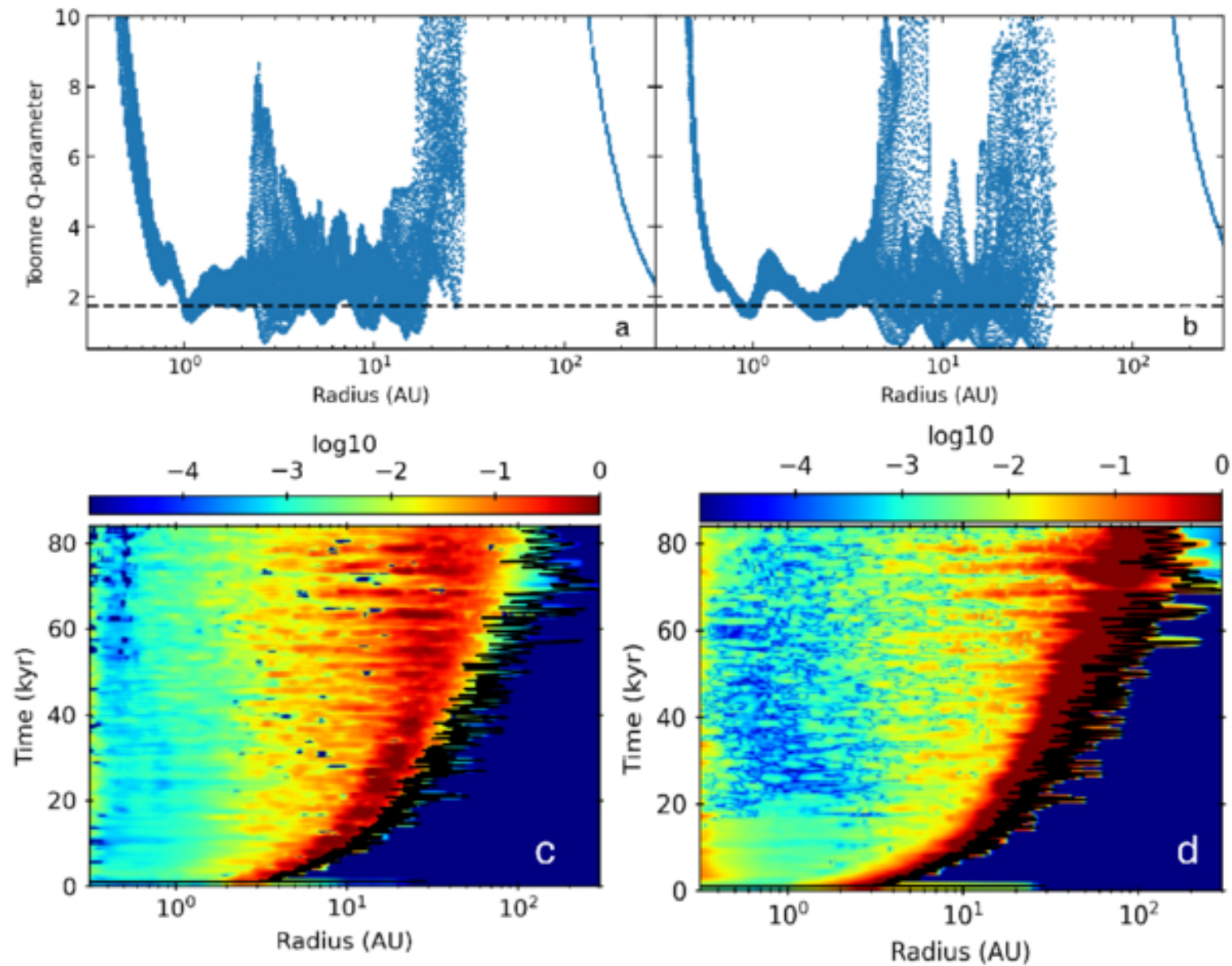
Figure 2. from Eduard I. Vorobyov et al 2026 Astrophys. J. Lett. 1007 doi:10.3847/2041-8213/ae907c https://dx.doi.org/10.3847/2041-8213/ae907c © 2026. The Author(s). Published by the American Astronomical Society.
